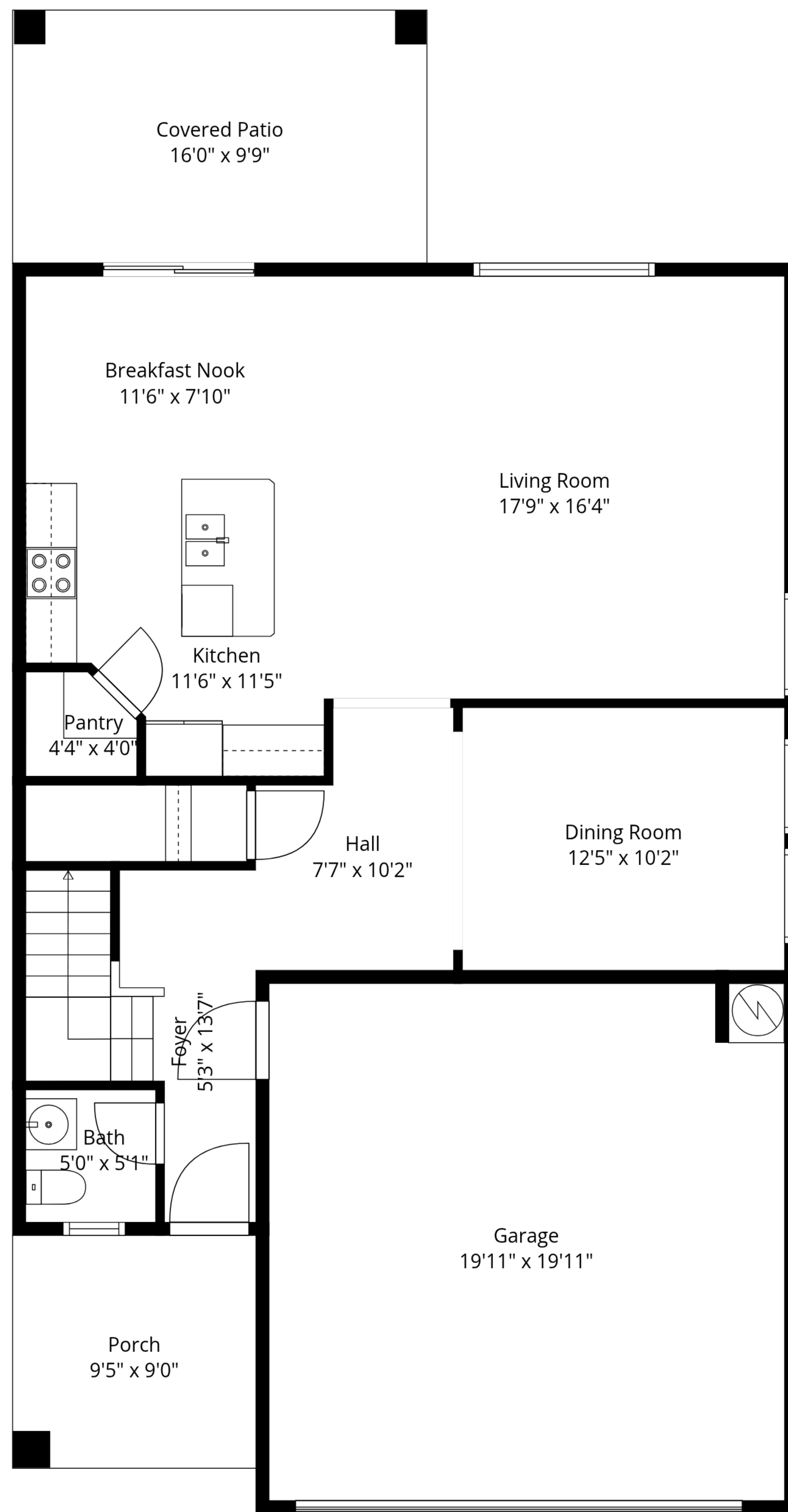
Floor 1
