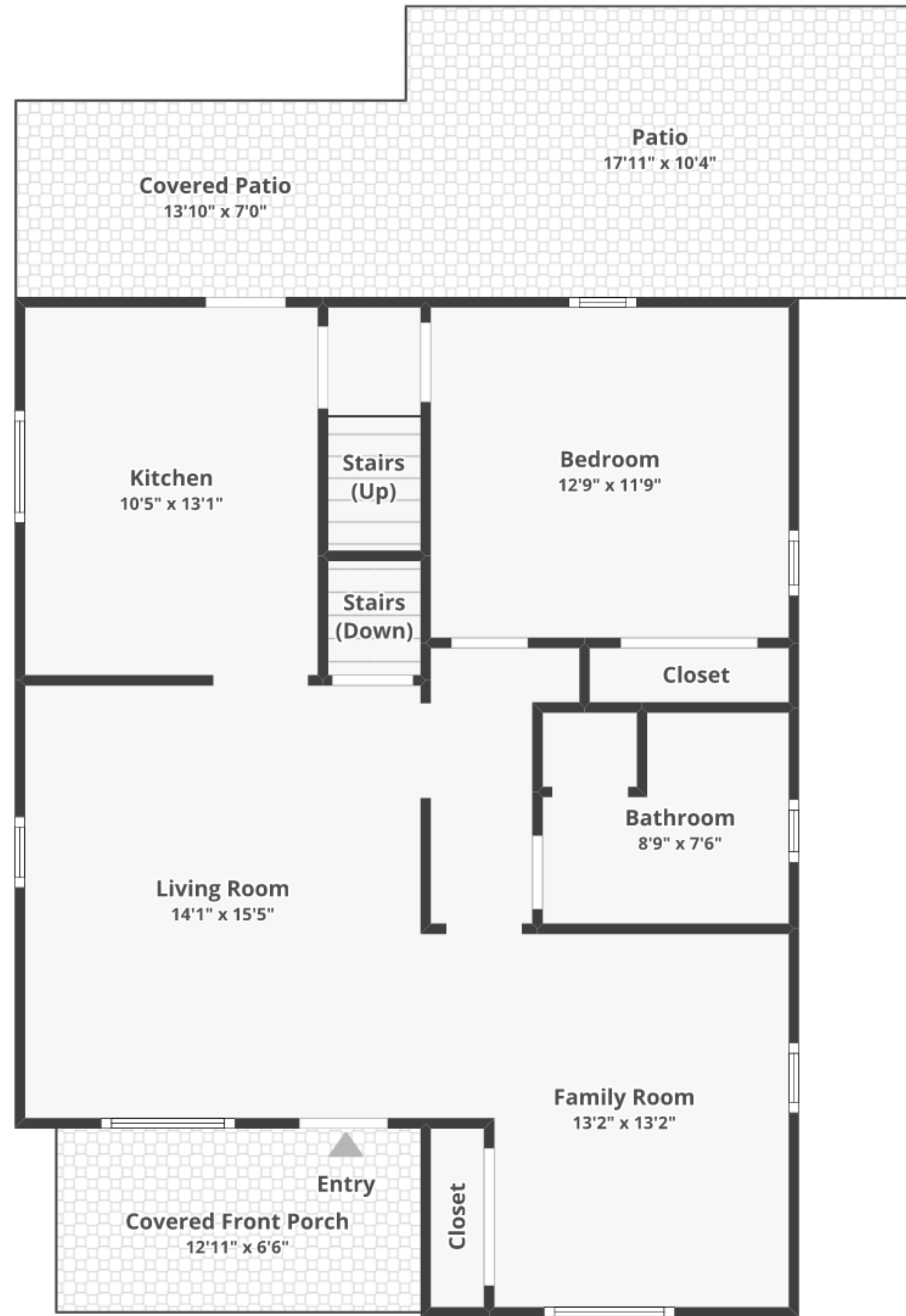
FLOOR 1
