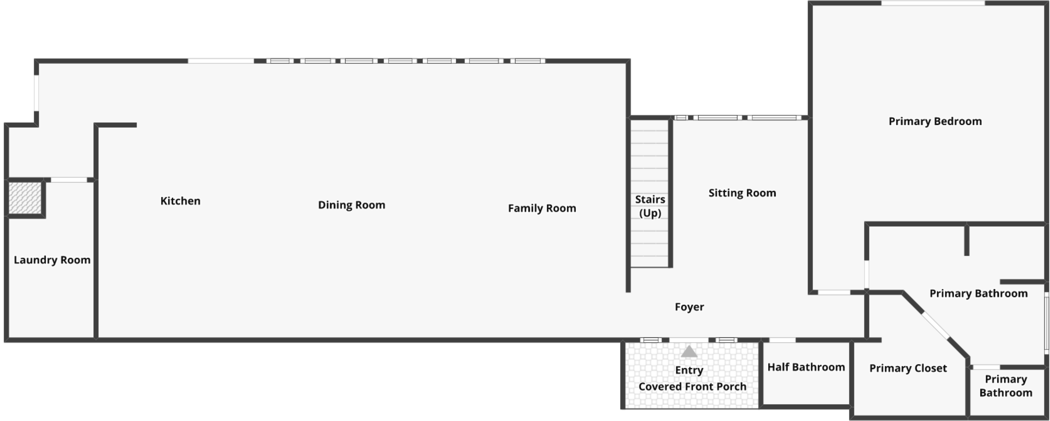
FLOOR 1
