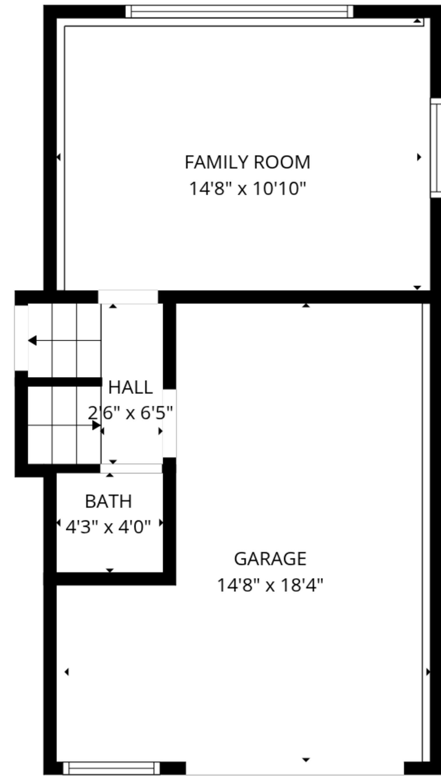
2nd floor
