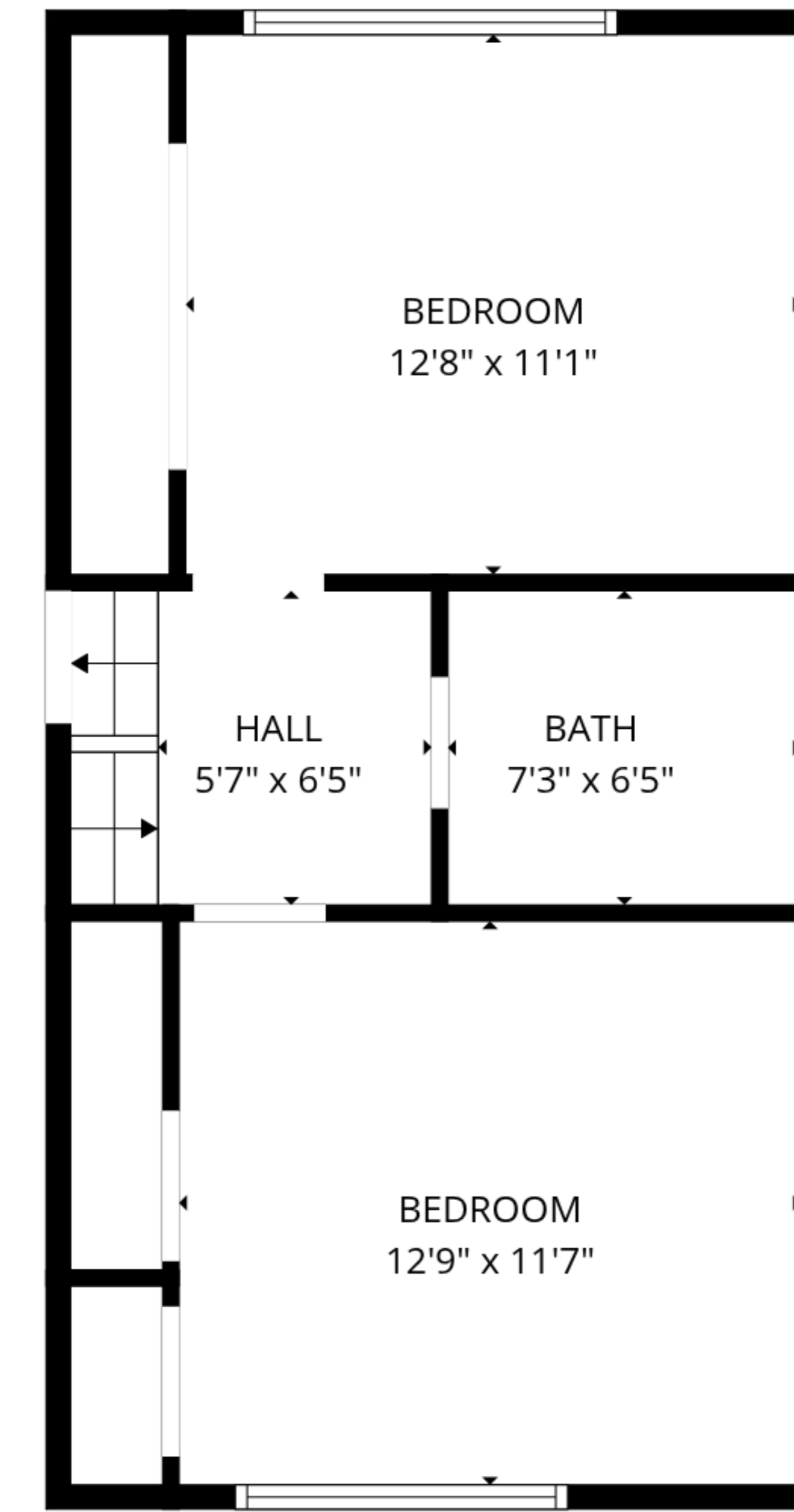
4th floor
