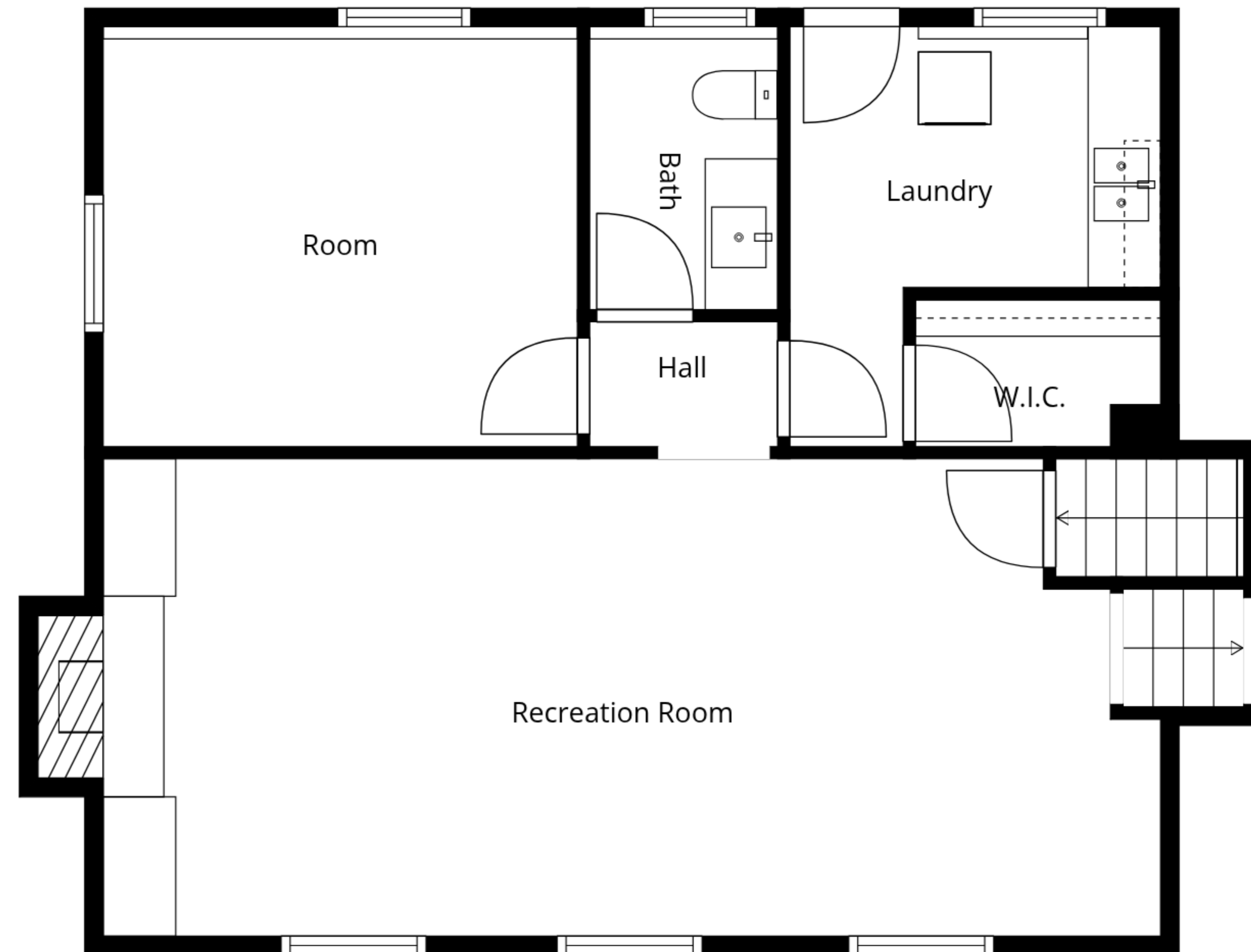
1st Floor
