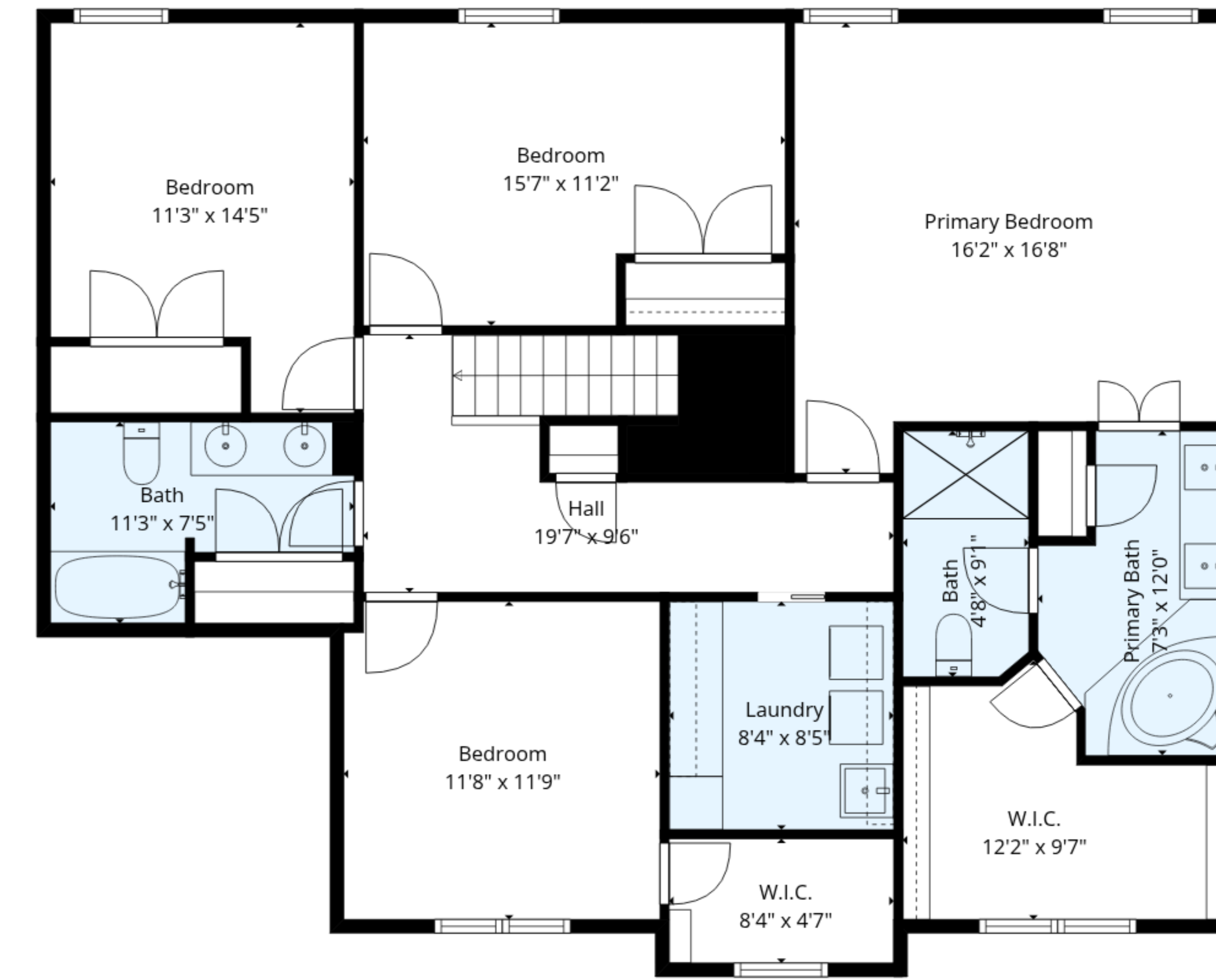
2nd Floor
