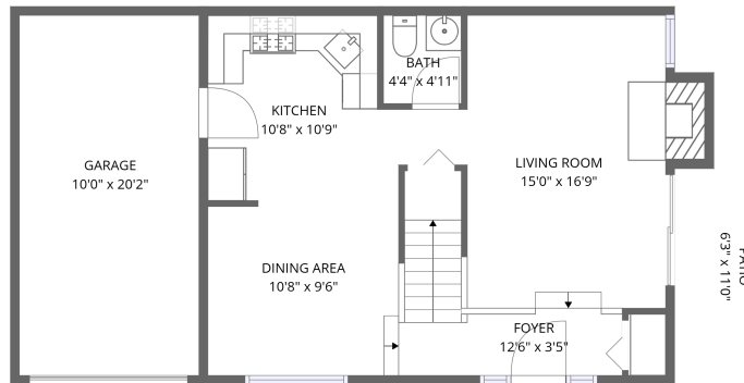
1st floor
