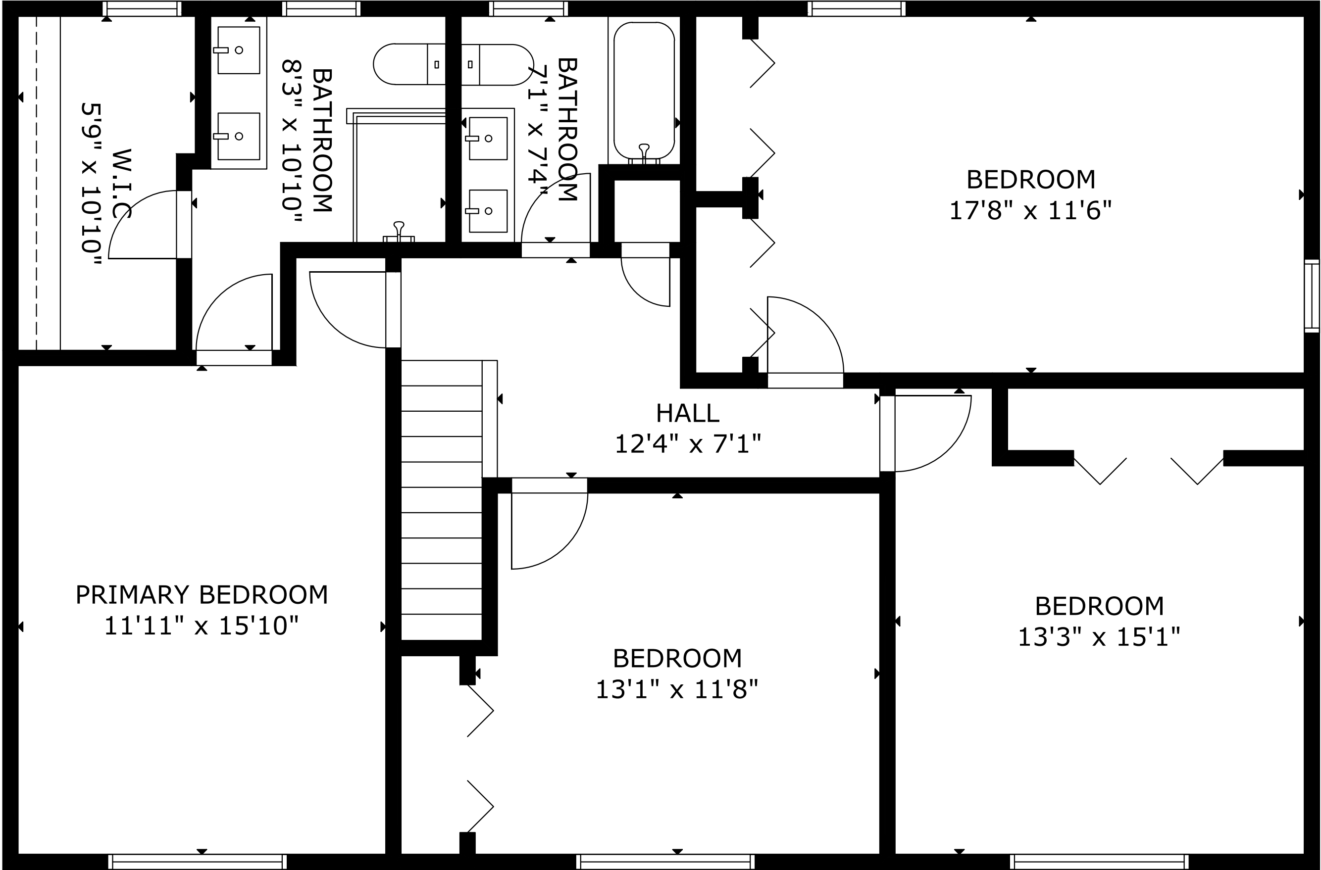
SECOND FLOOR
