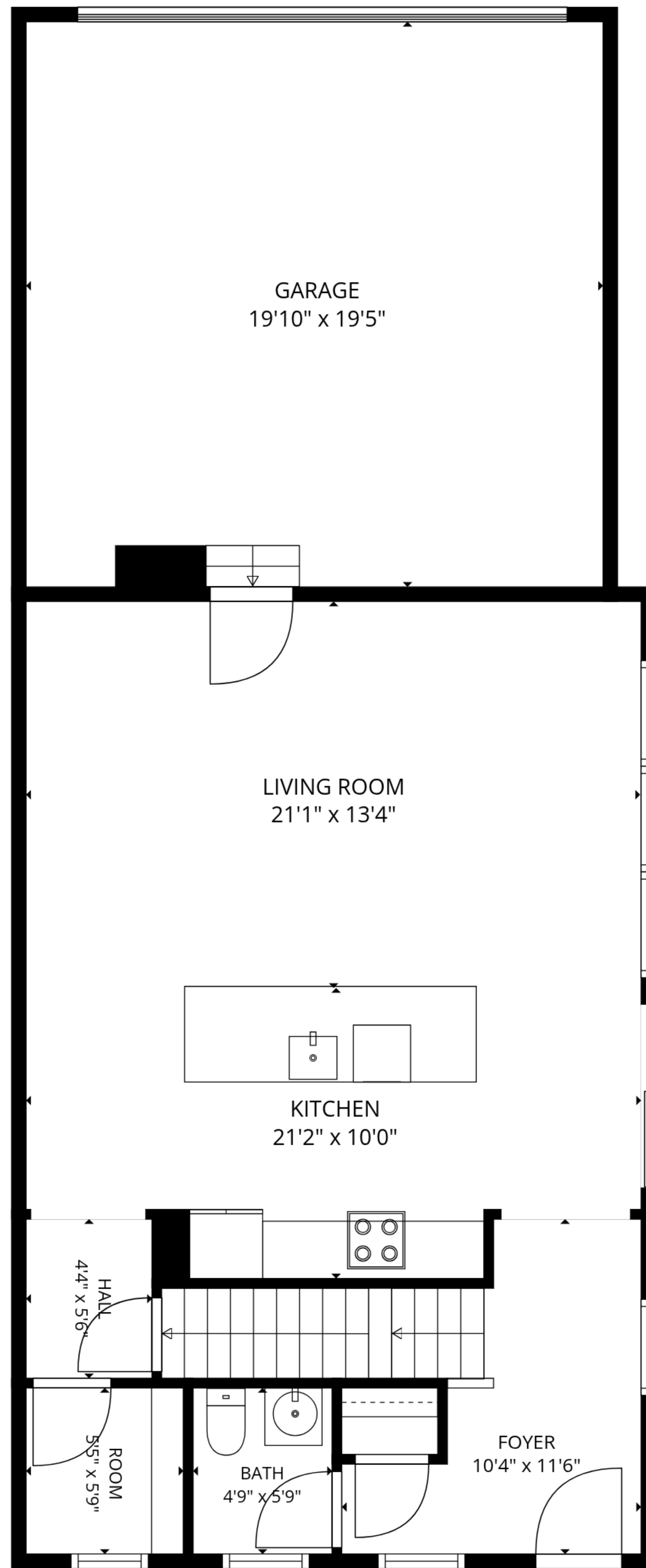
1st floor
