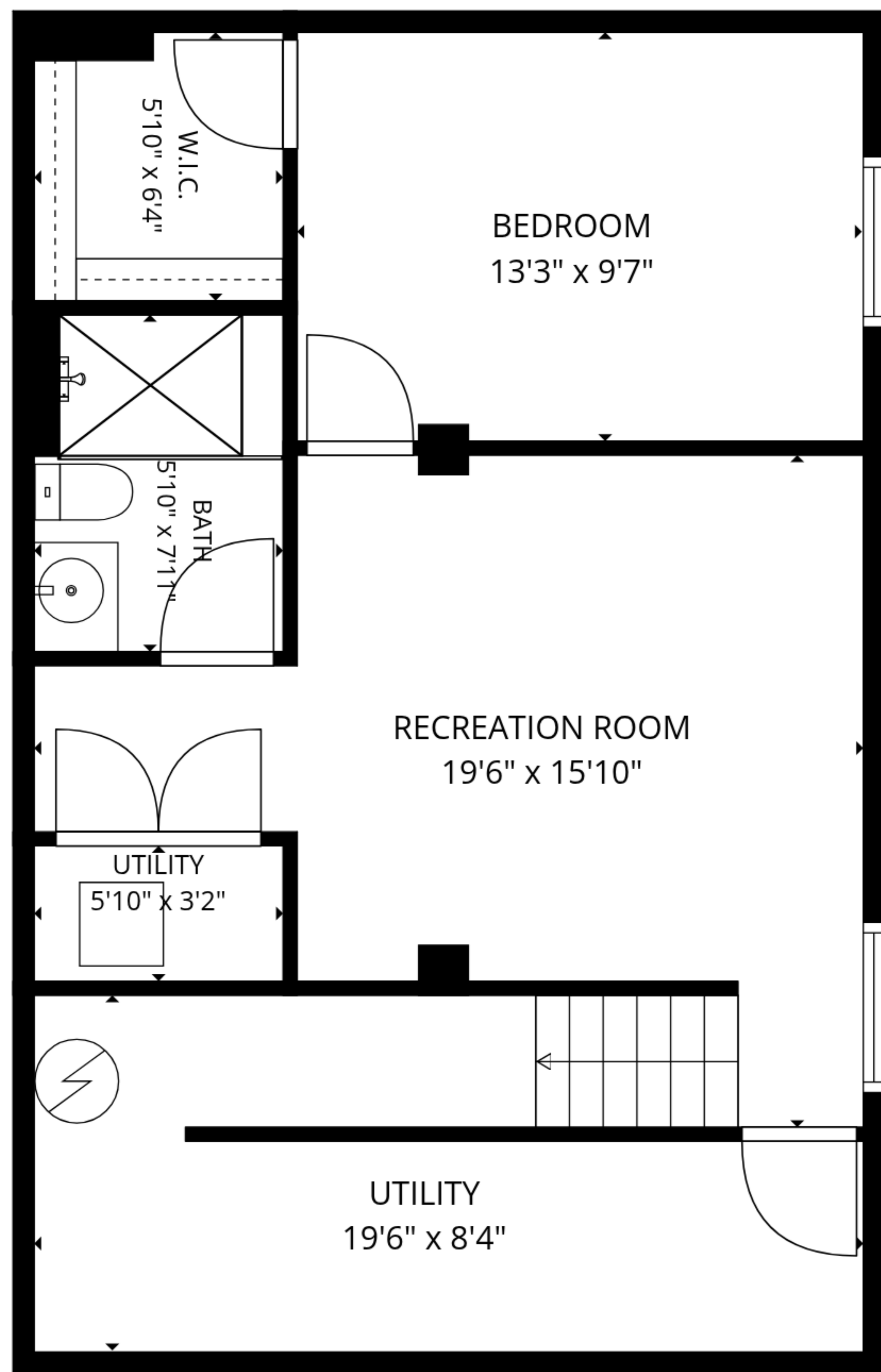
Basement
