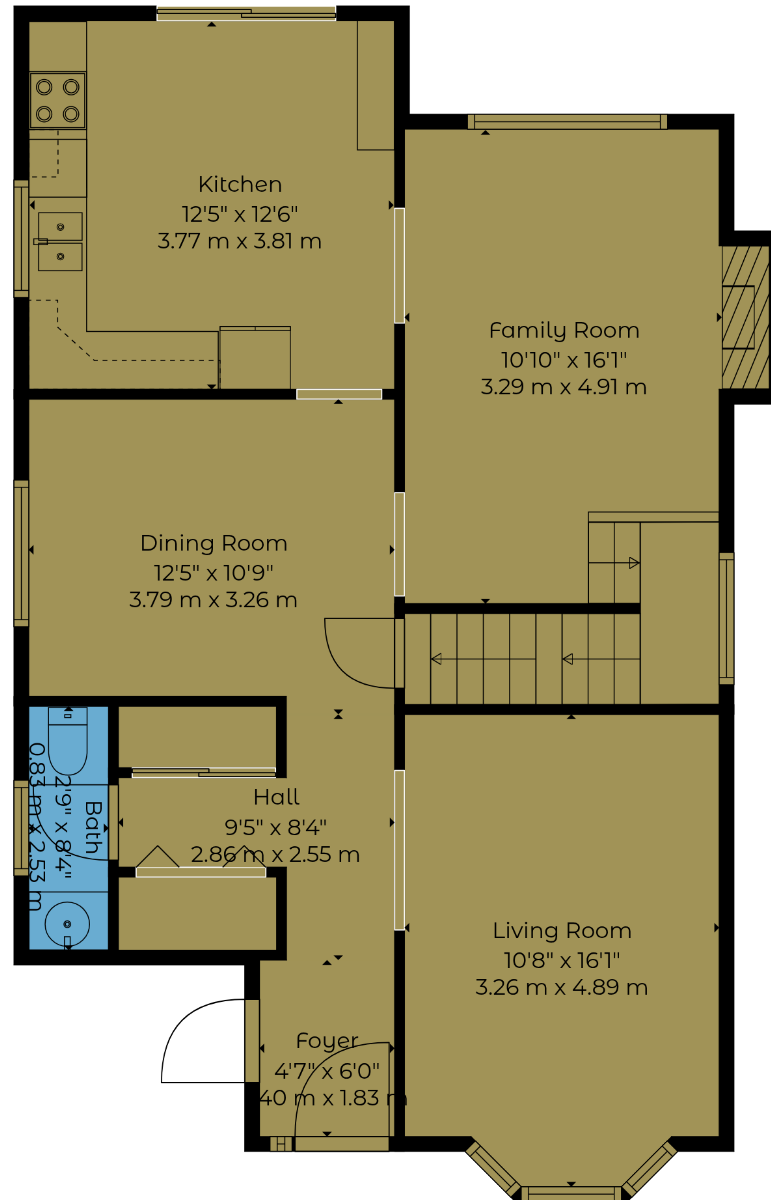
Floor 2
