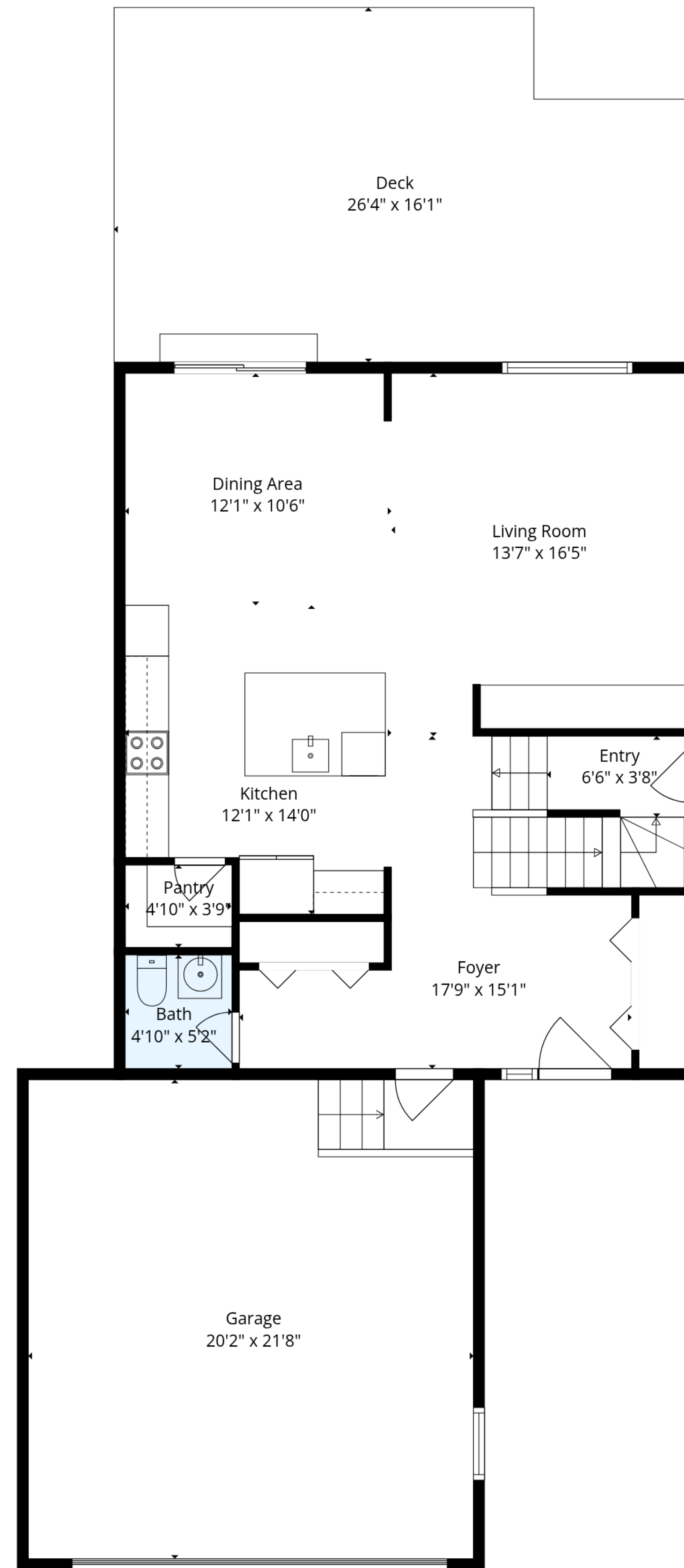
1st Floor
