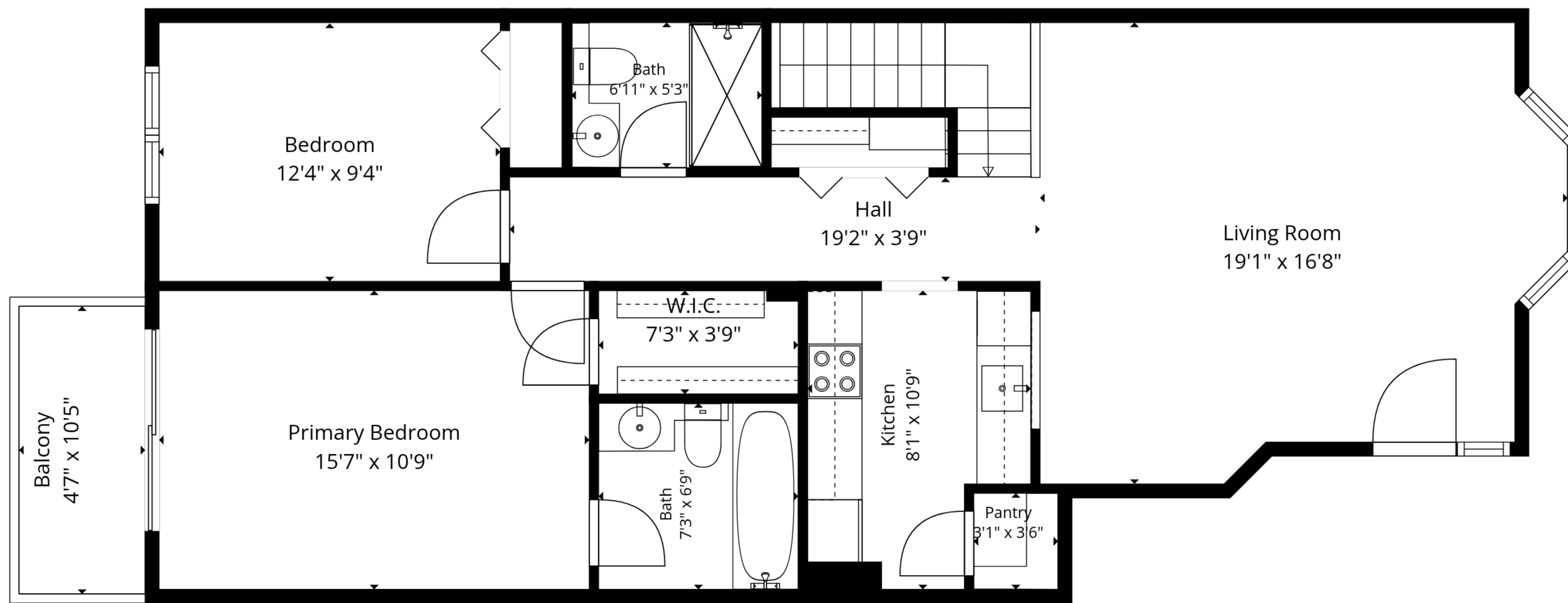
2nd Floor
