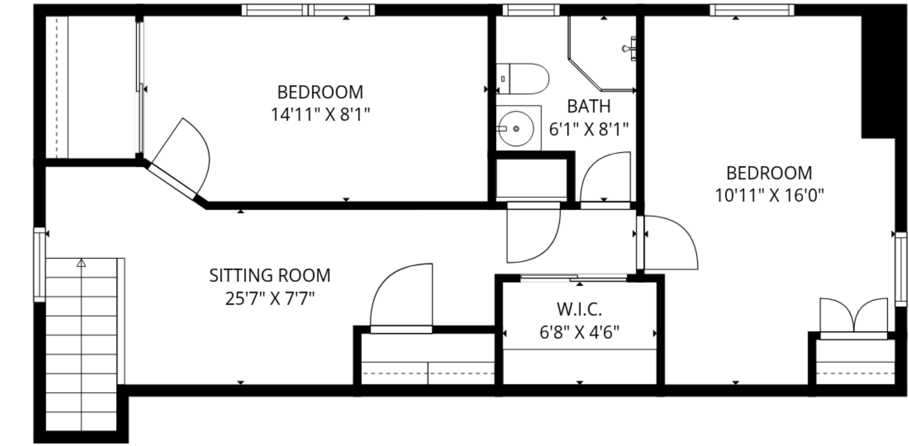
SECOND FLOOR
