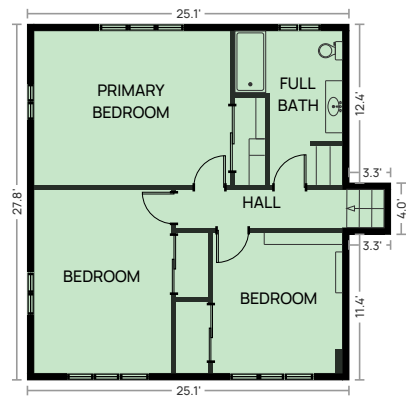
SECOND FLOOR Above grade - 8'4" ceiling - GLA 710 sq ft
