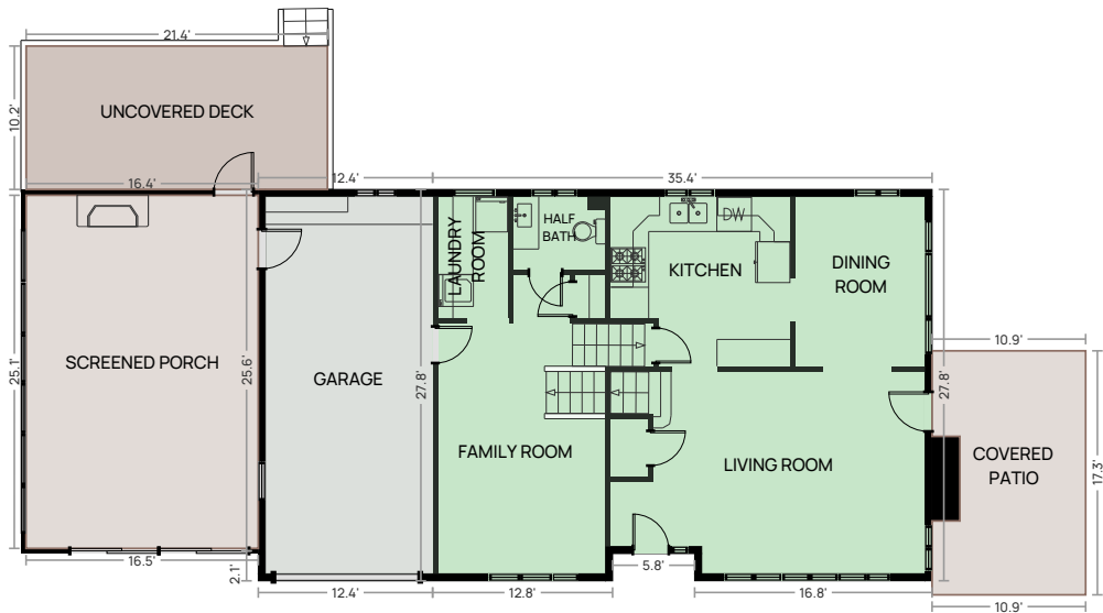
FIRST FLOOR Above grade - 8'8" ceiling - GLA 972 sq ft
