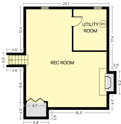
BASEMENT Below grade - 8'6" ceiling - Finished 644 sq ft
