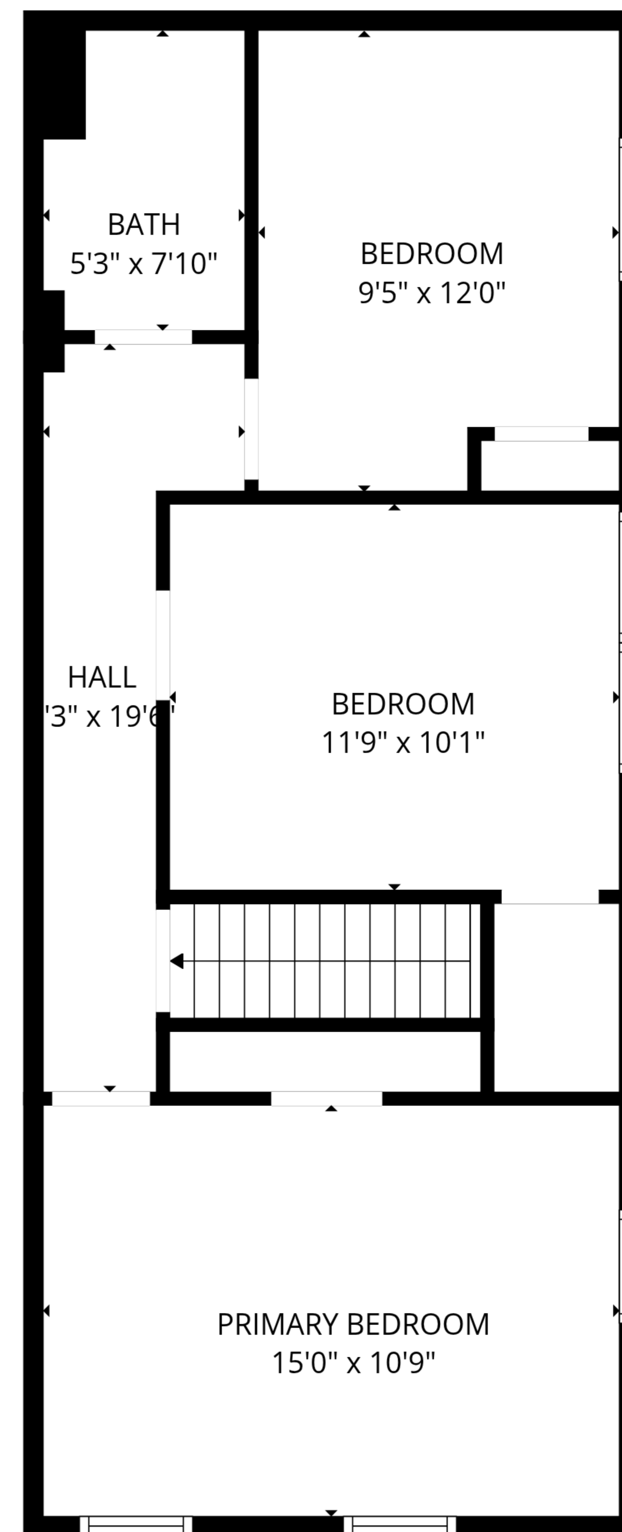
2RD FLOOR
