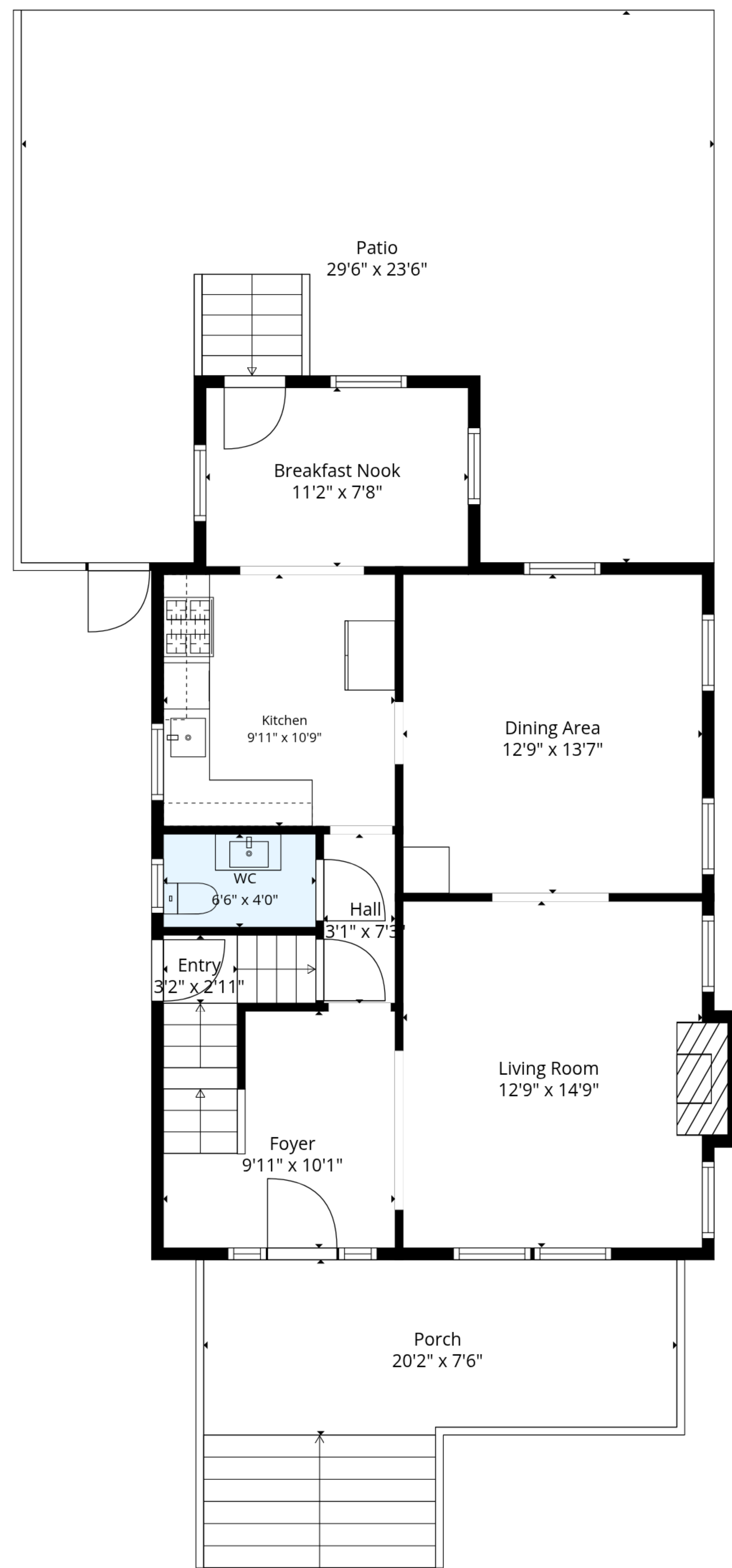
Ground Floor
