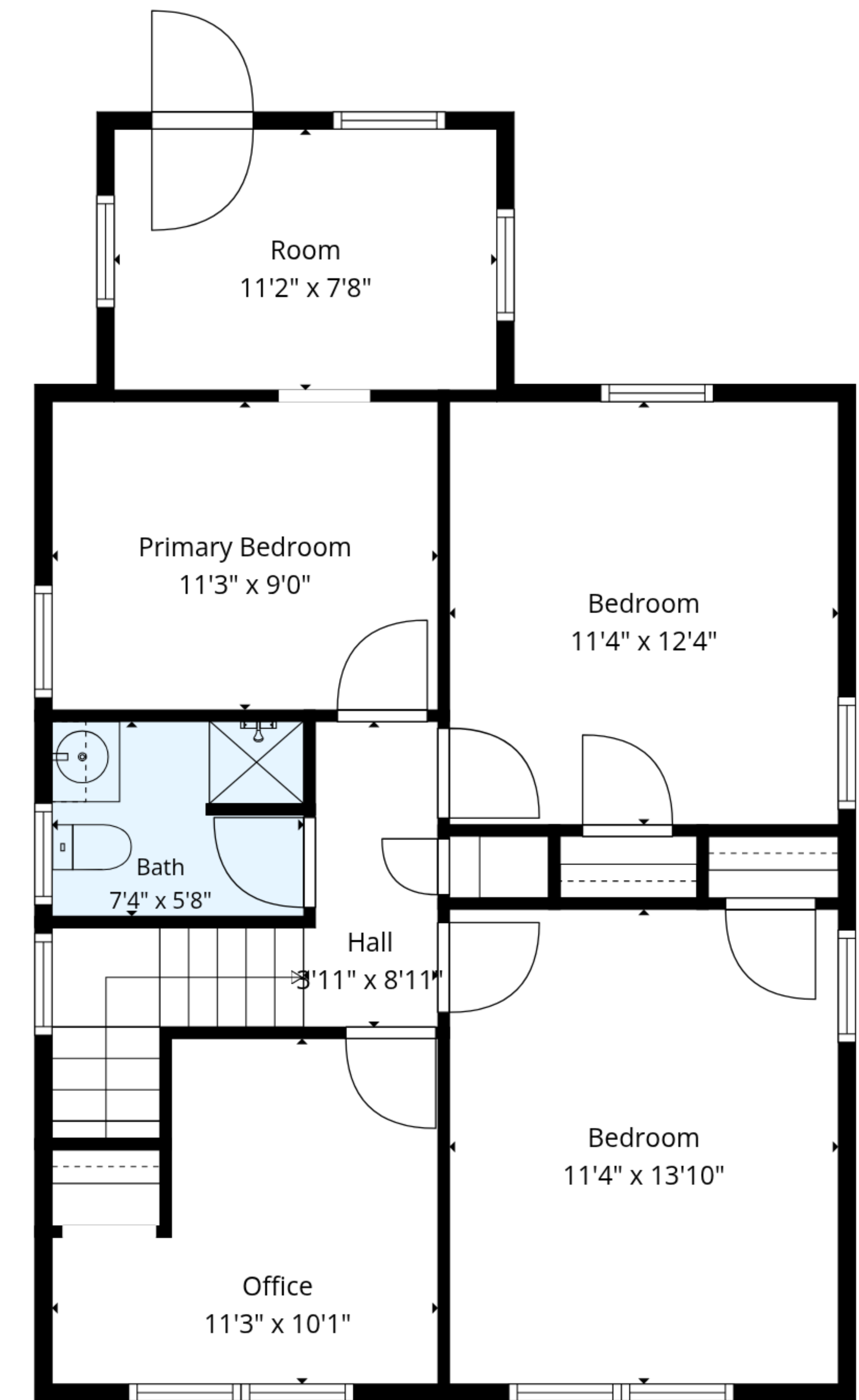
1st Floor
