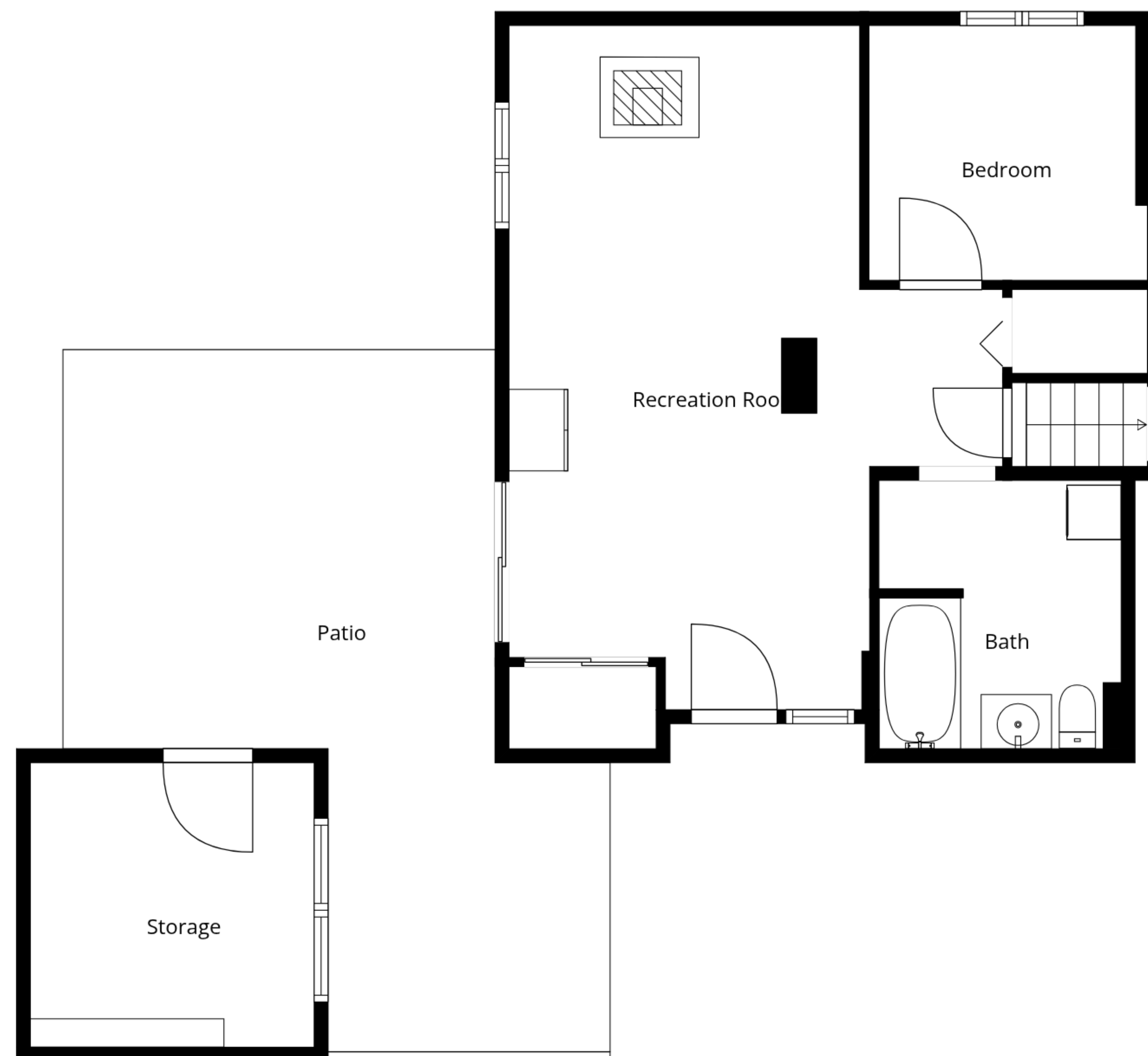
1st Floor
