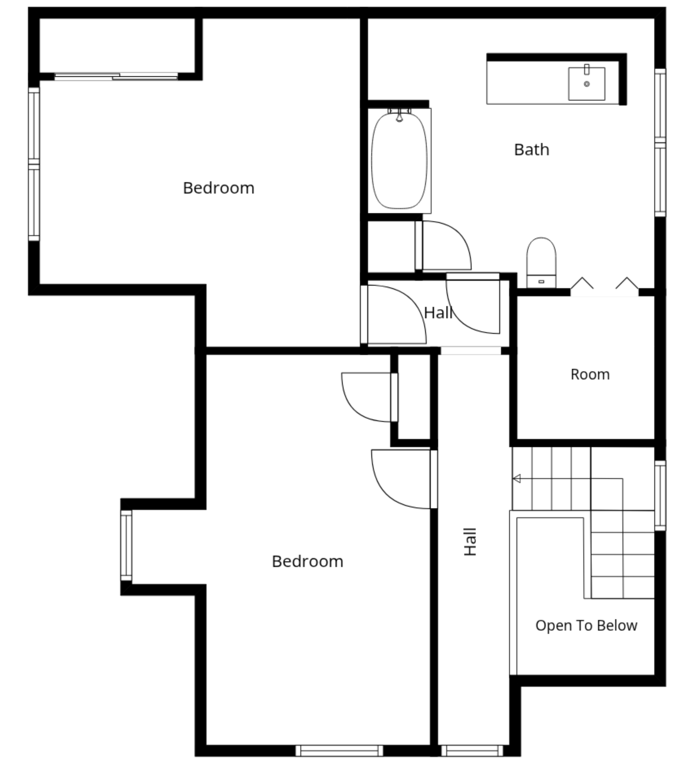
3rd Floor
