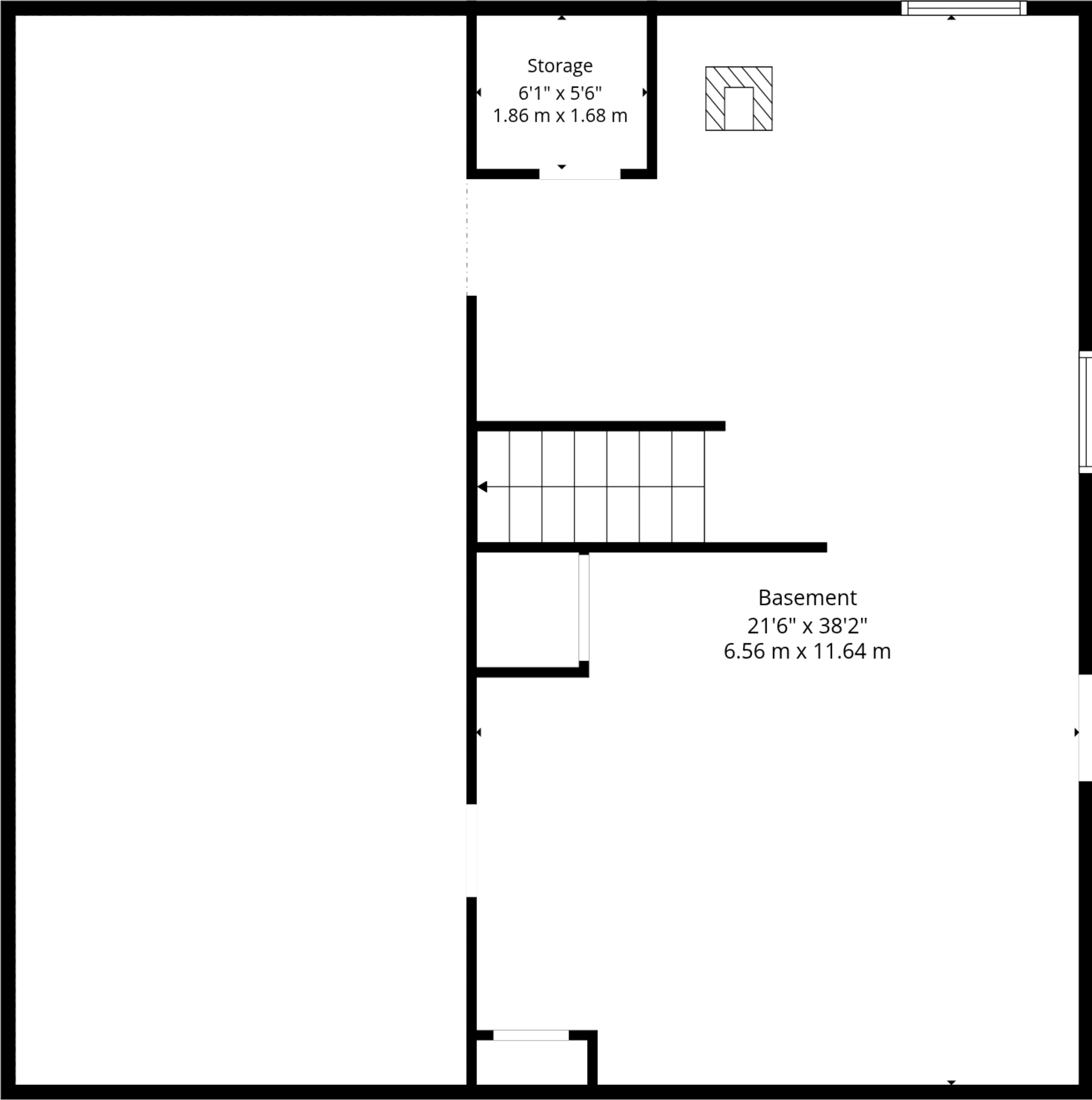
Basement
