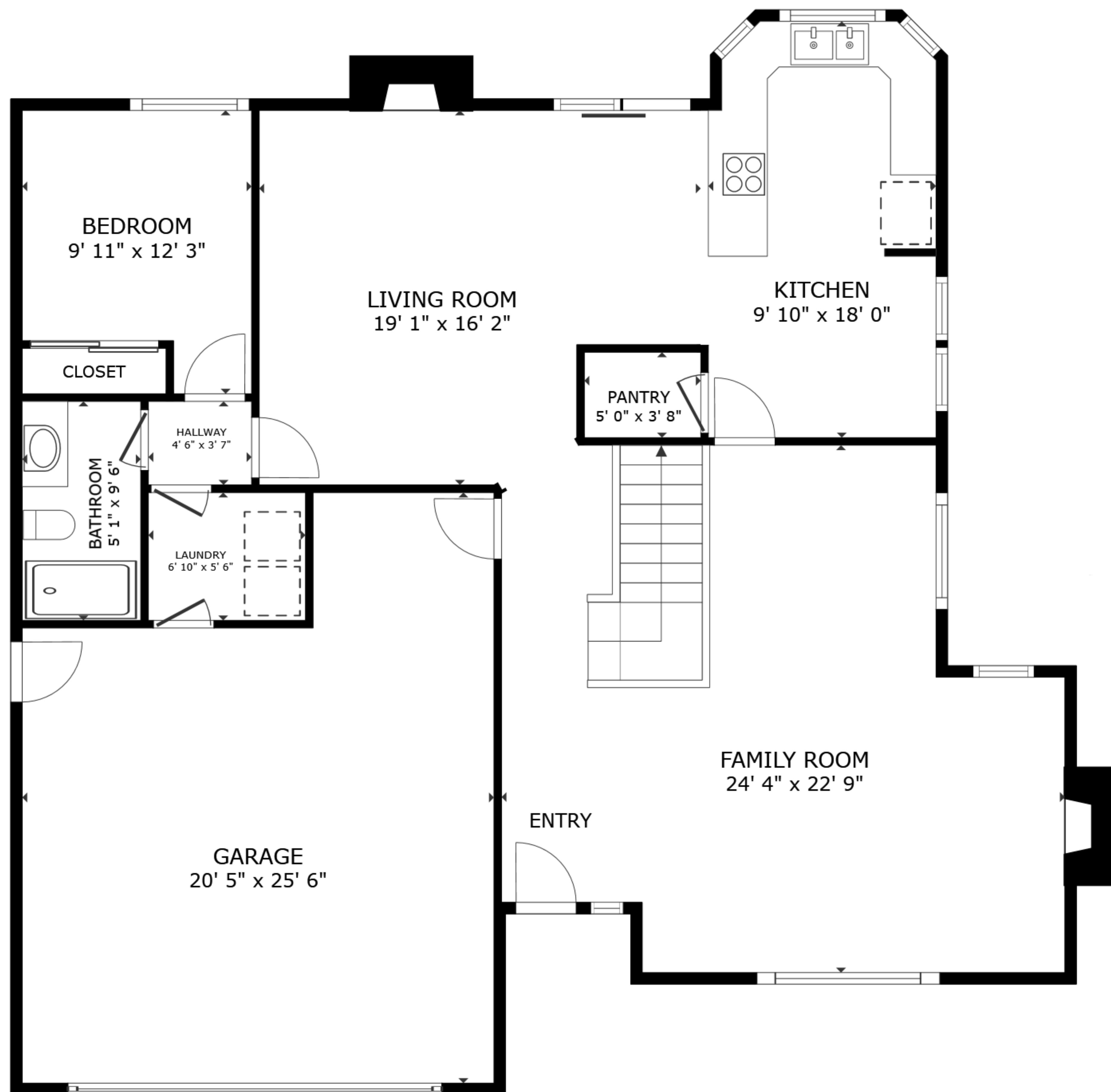
FLOOR 1
