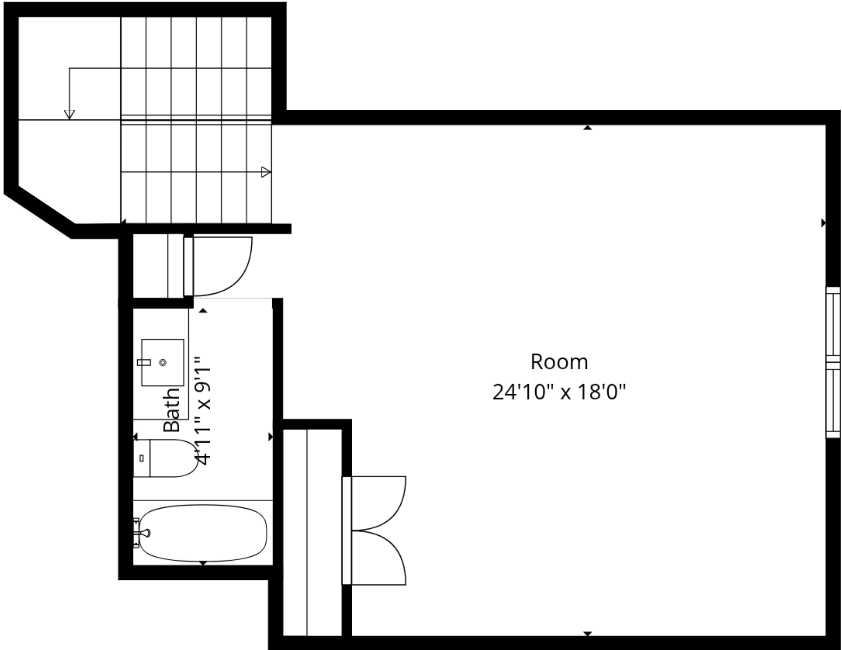
2nd Floor
