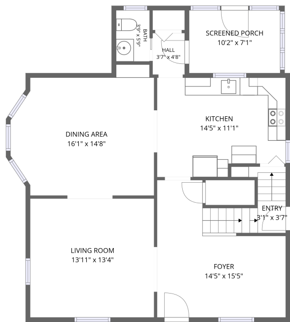
1st floor
