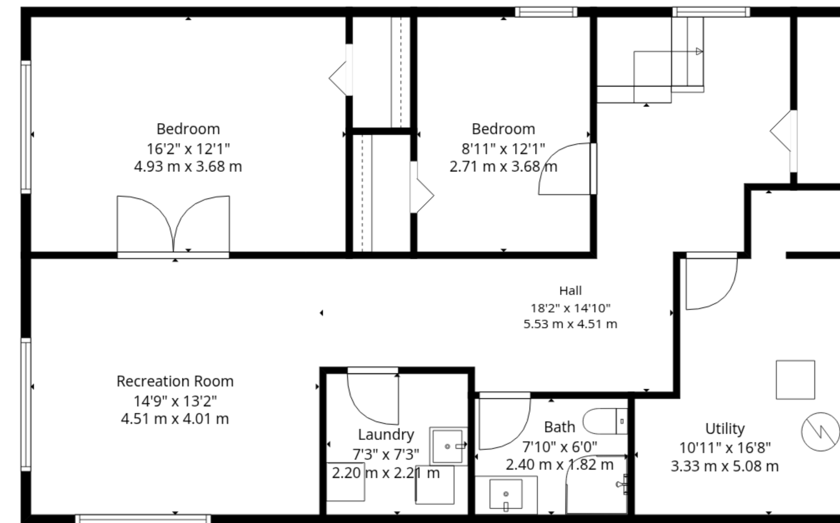
Basement
