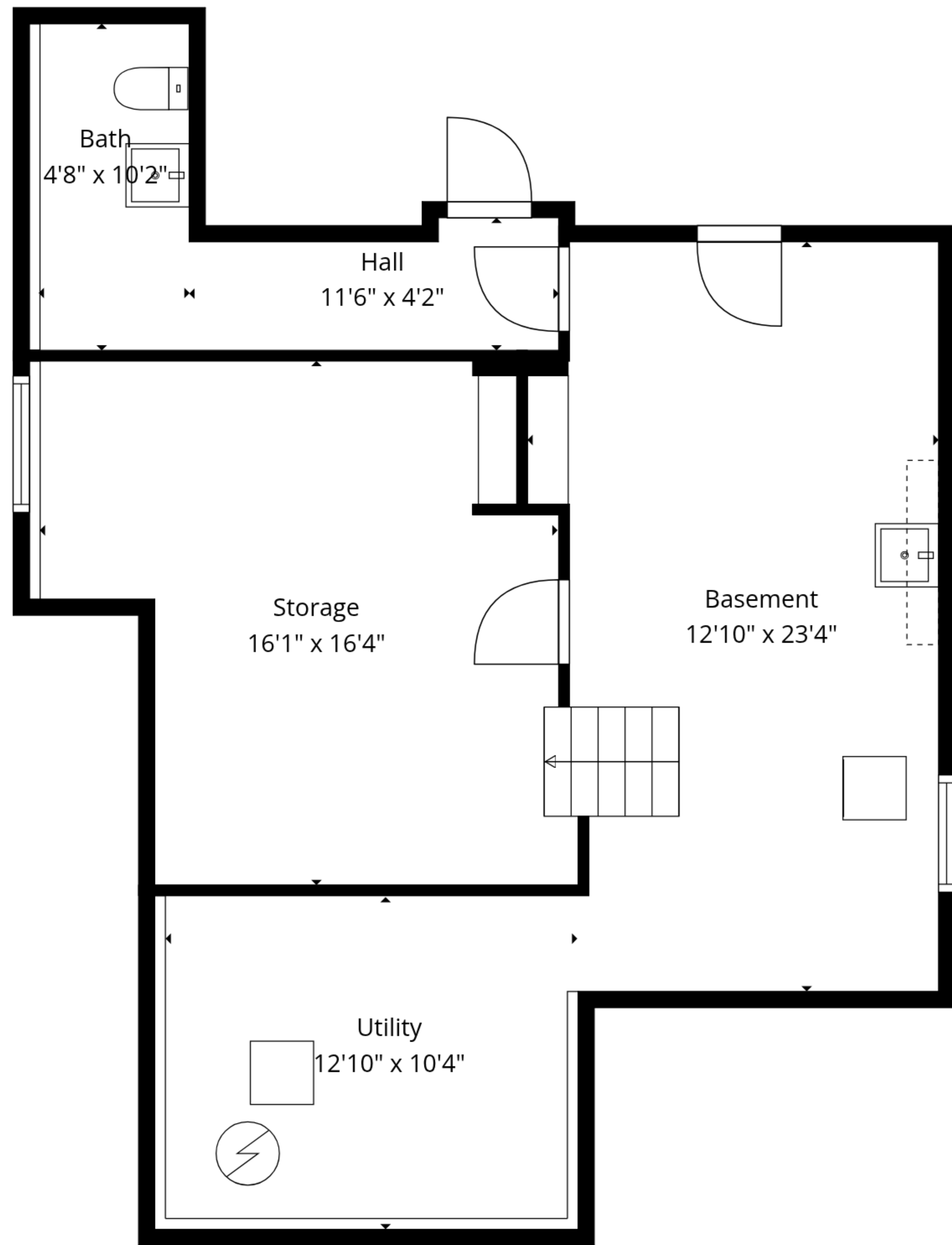
Basement
