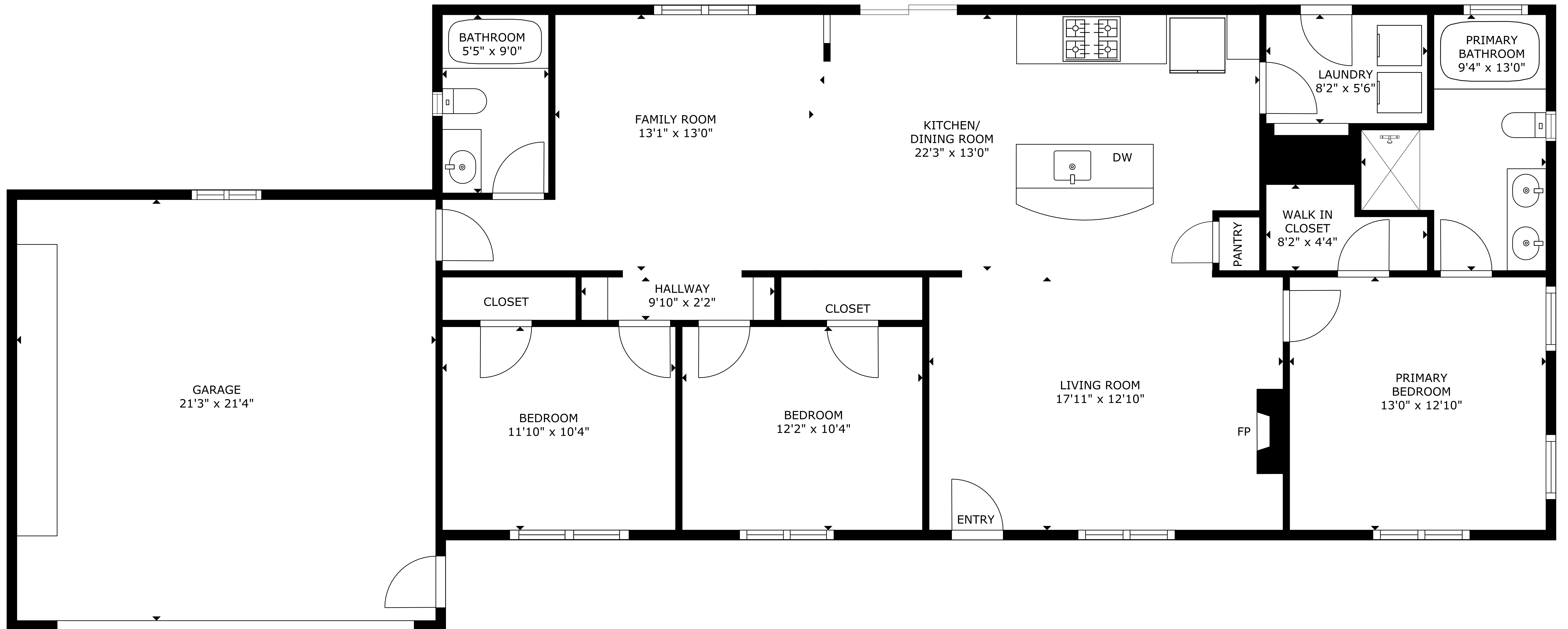
FLOOR PLAN
