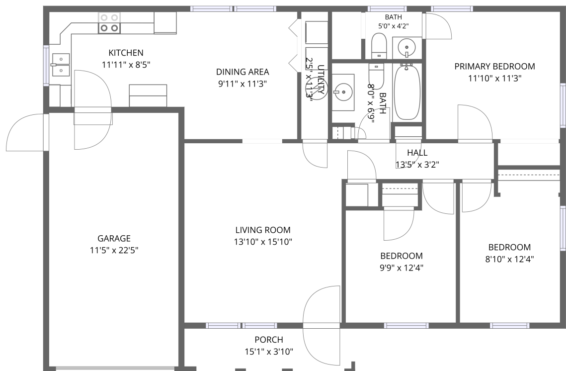
1st floor
