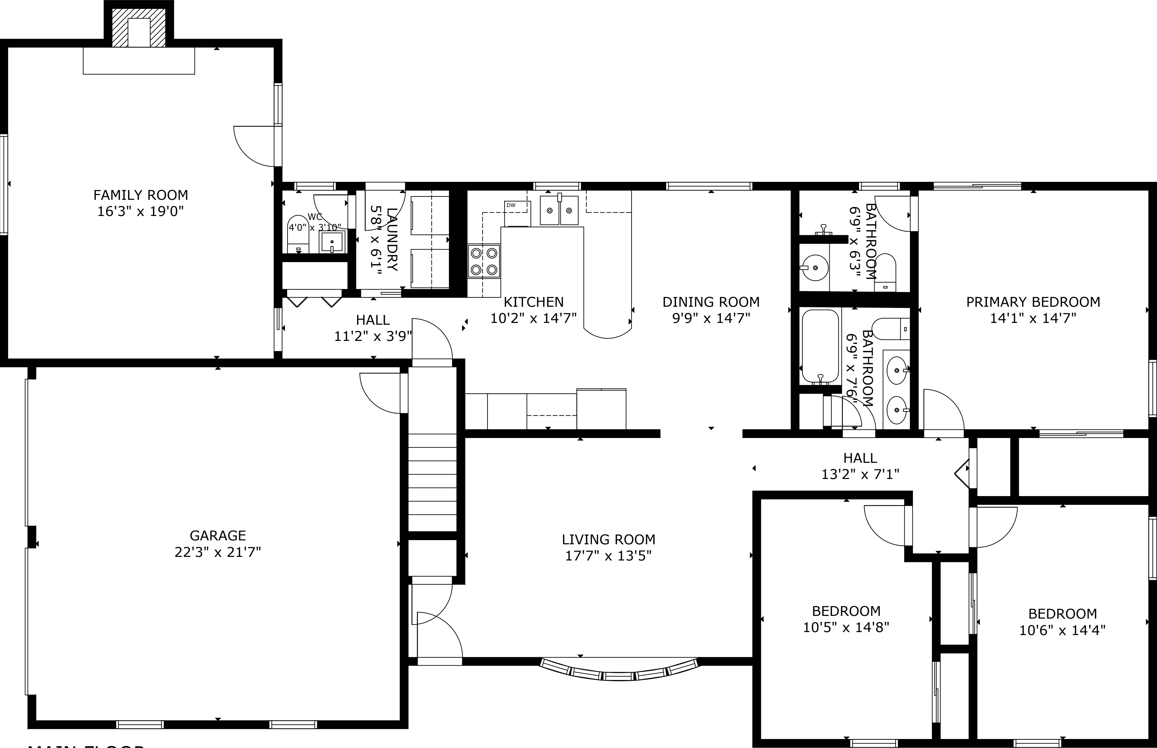
MAIN FLOOR
