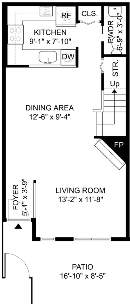
MAIN FLOOR 516 sq.ft. | Ceiling Height: 8'-0"
