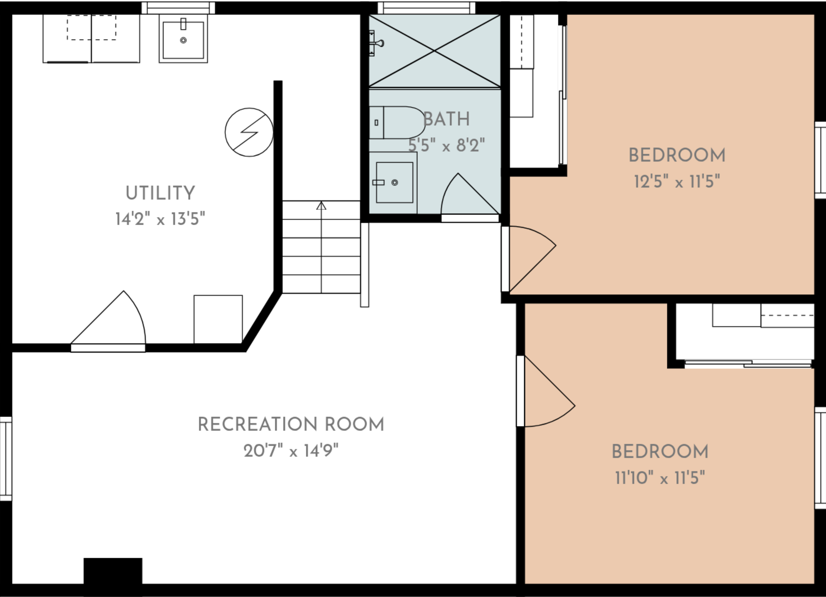
1st floor
