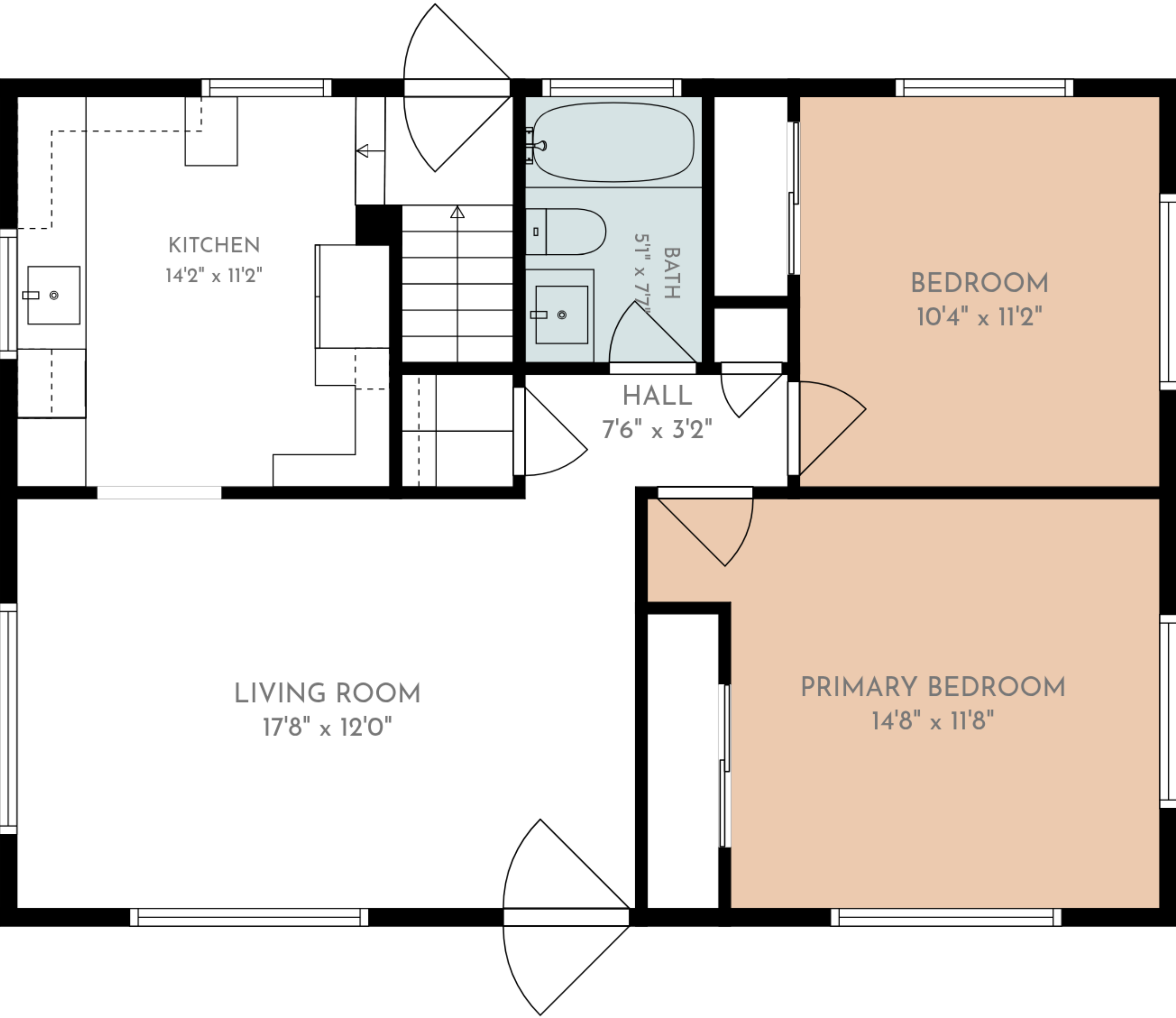
1st floor
