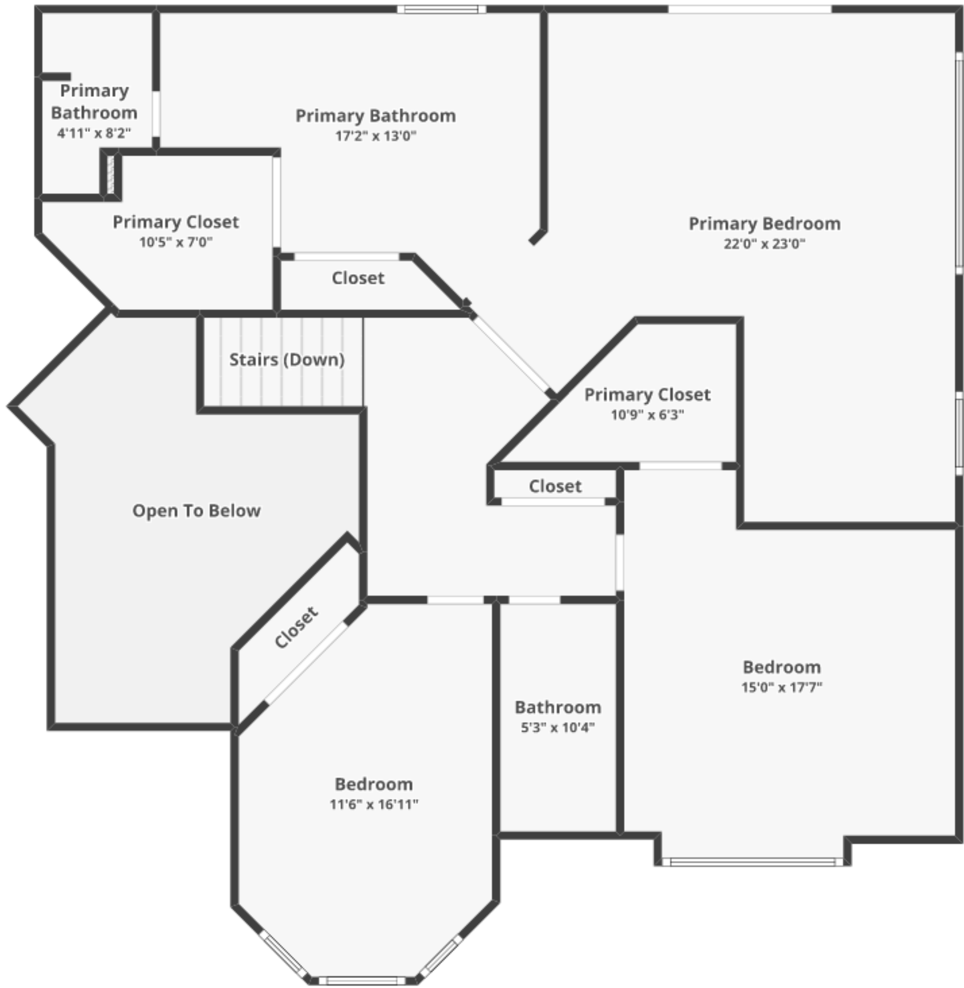
FLOOR 2
