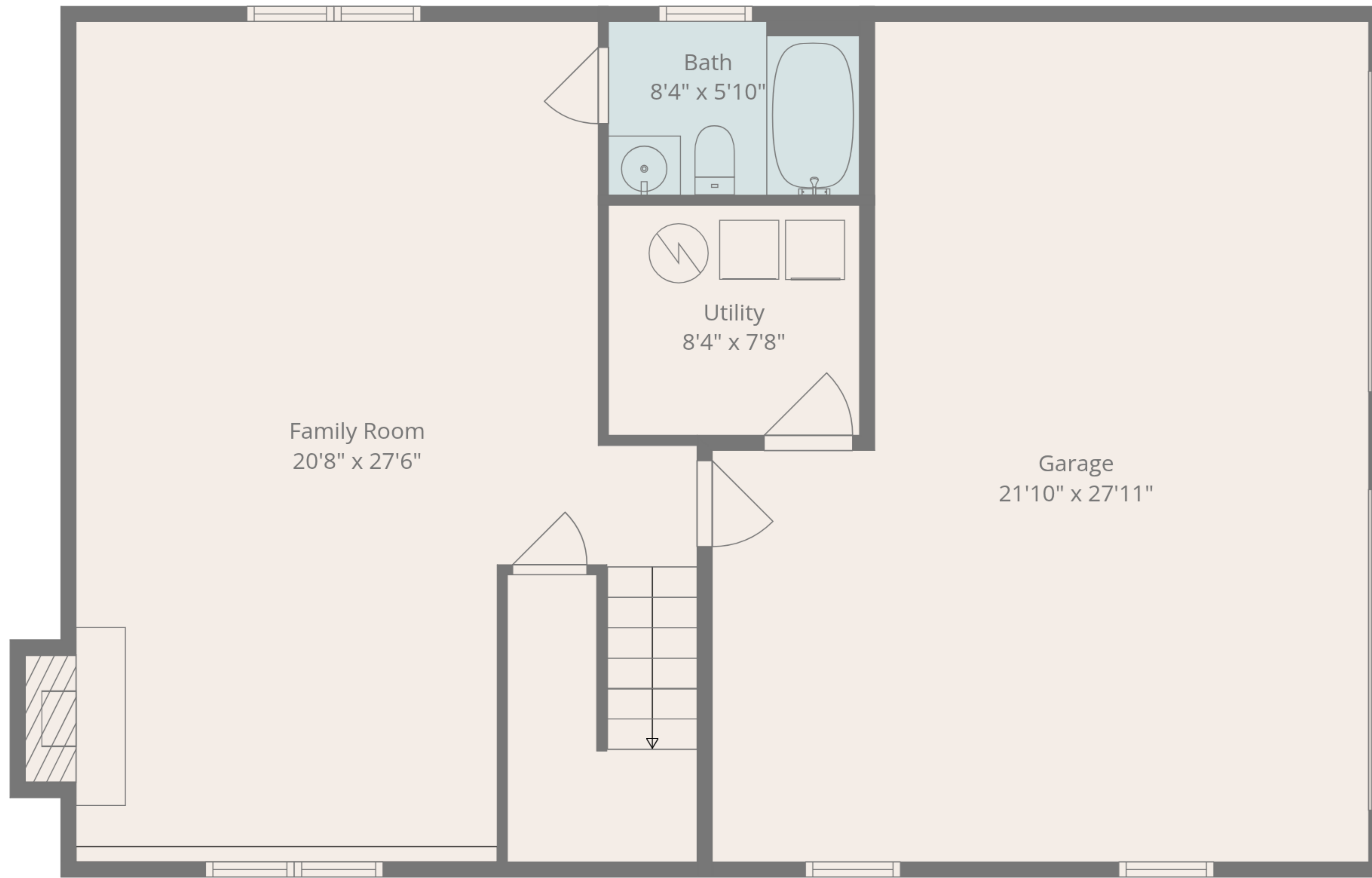
Basement
