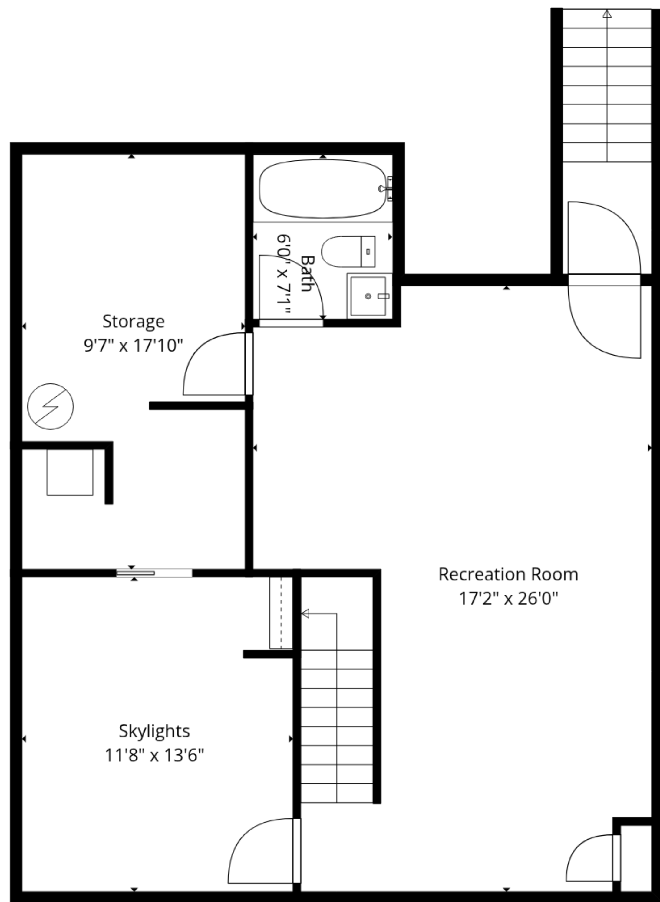
Basement
