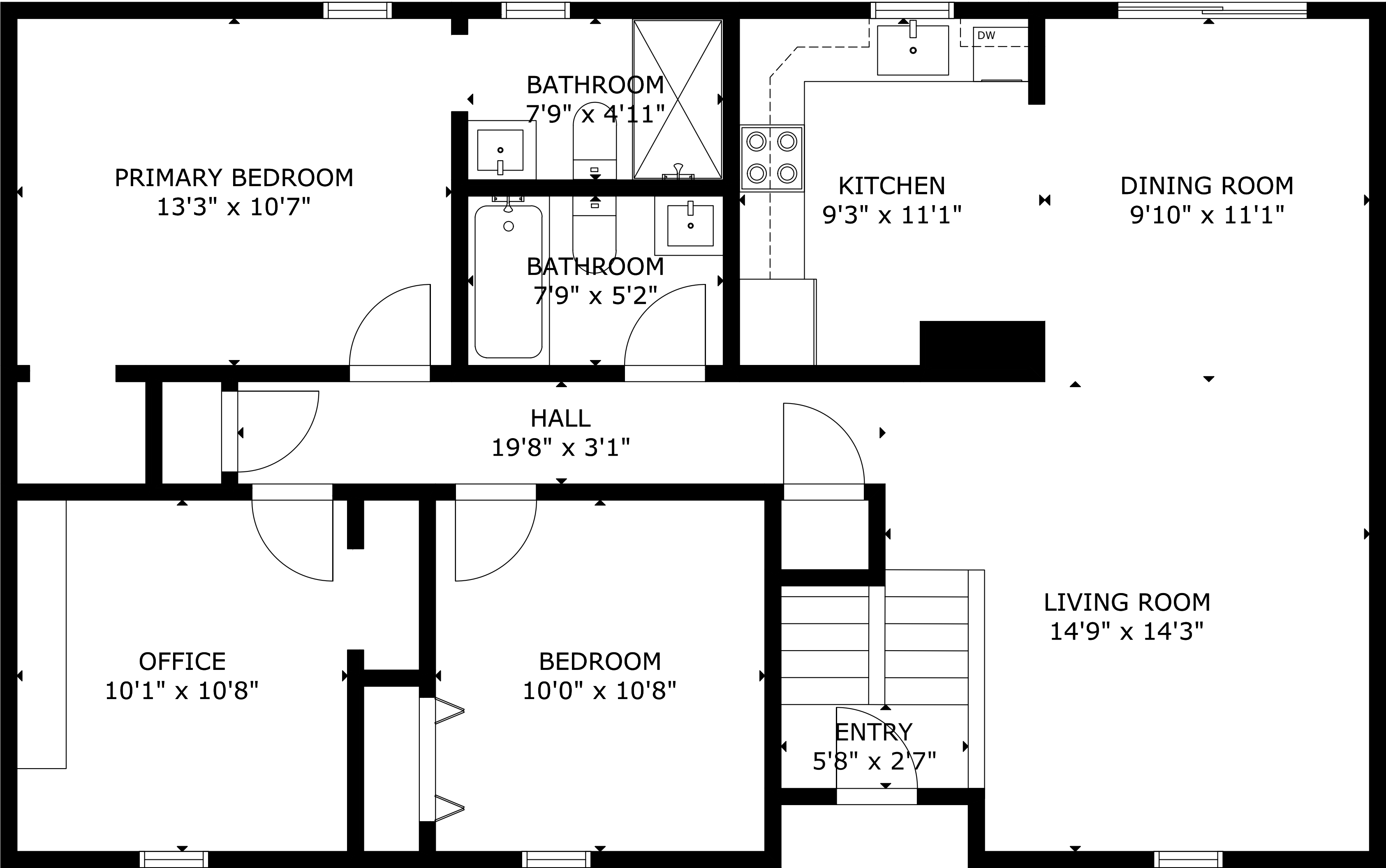
MAIN FLOOR
