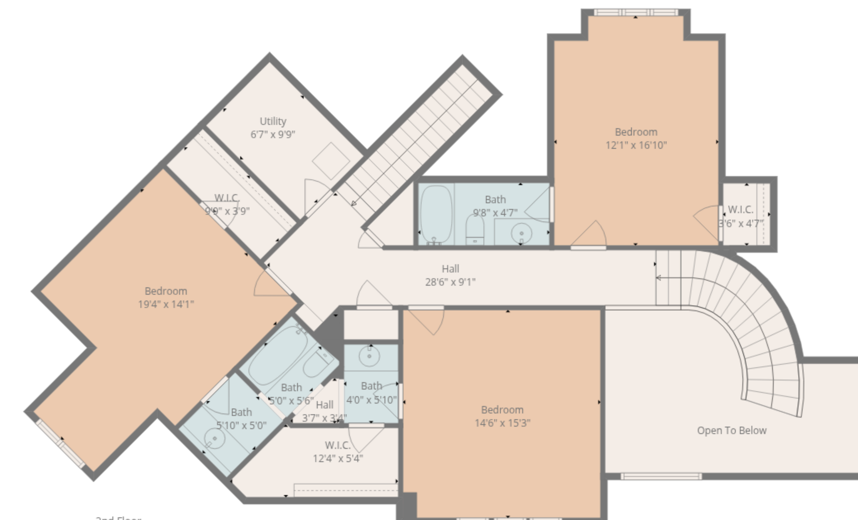
2nd Floor
