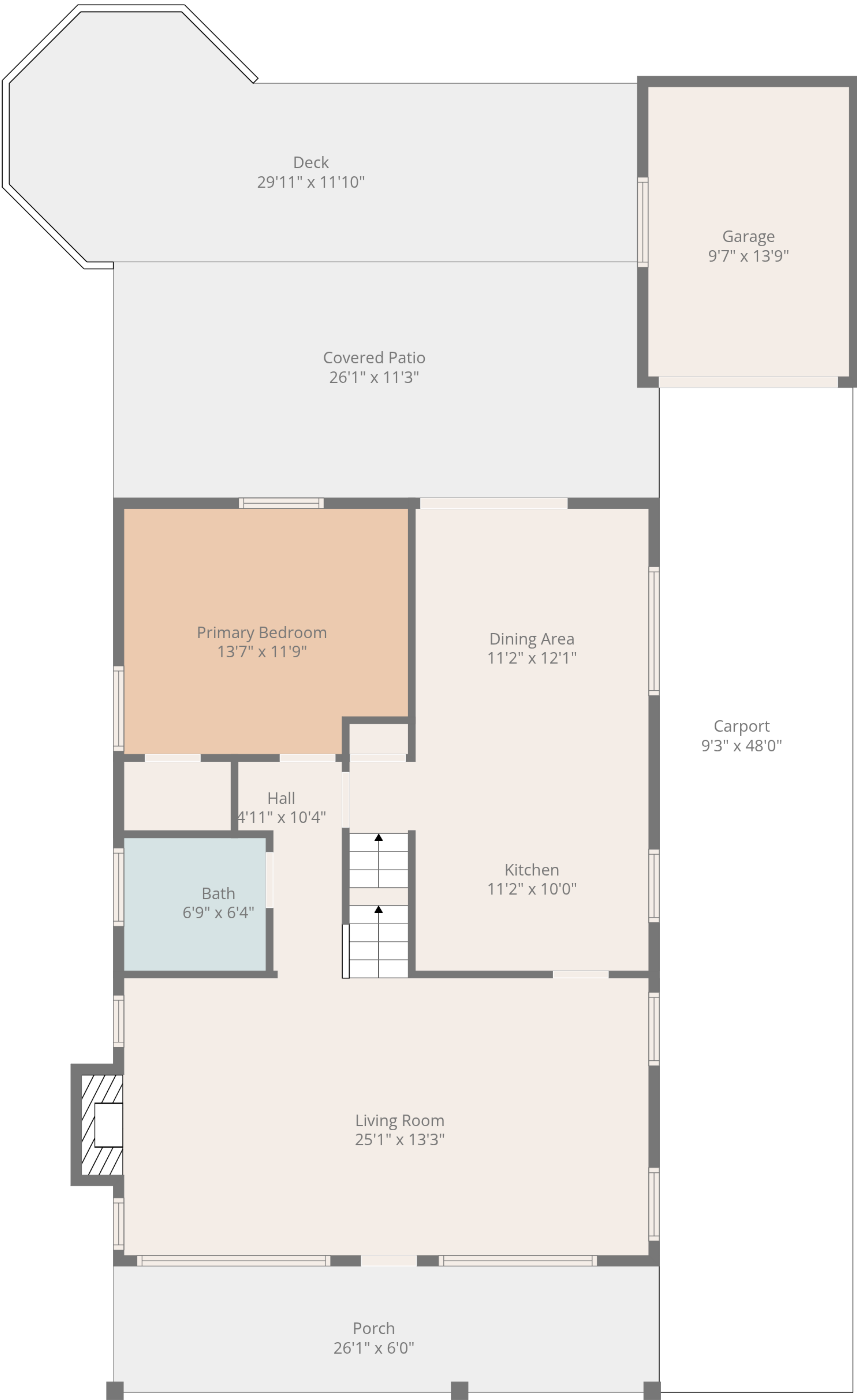
Floor 2
