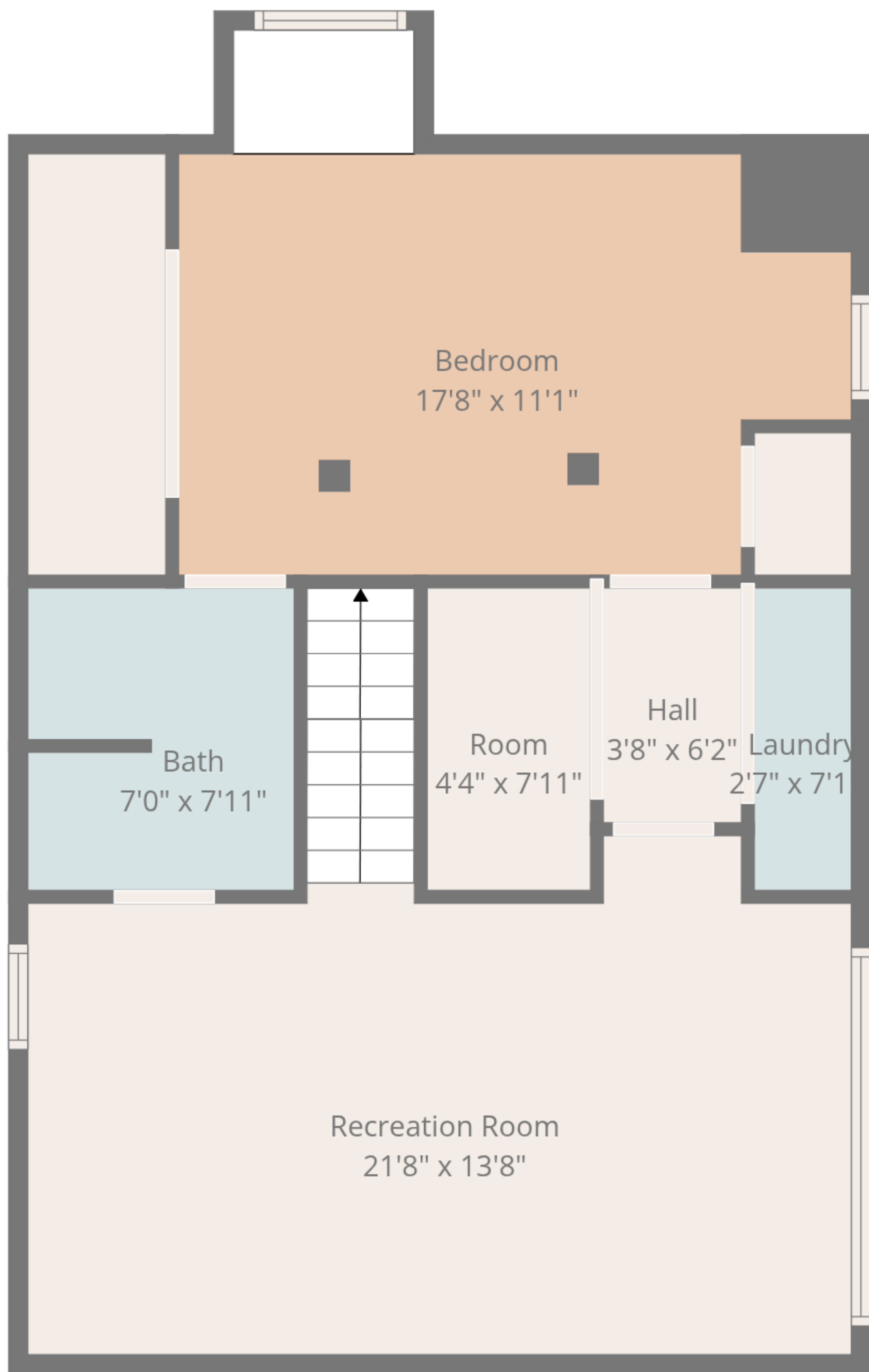
Floor 1
