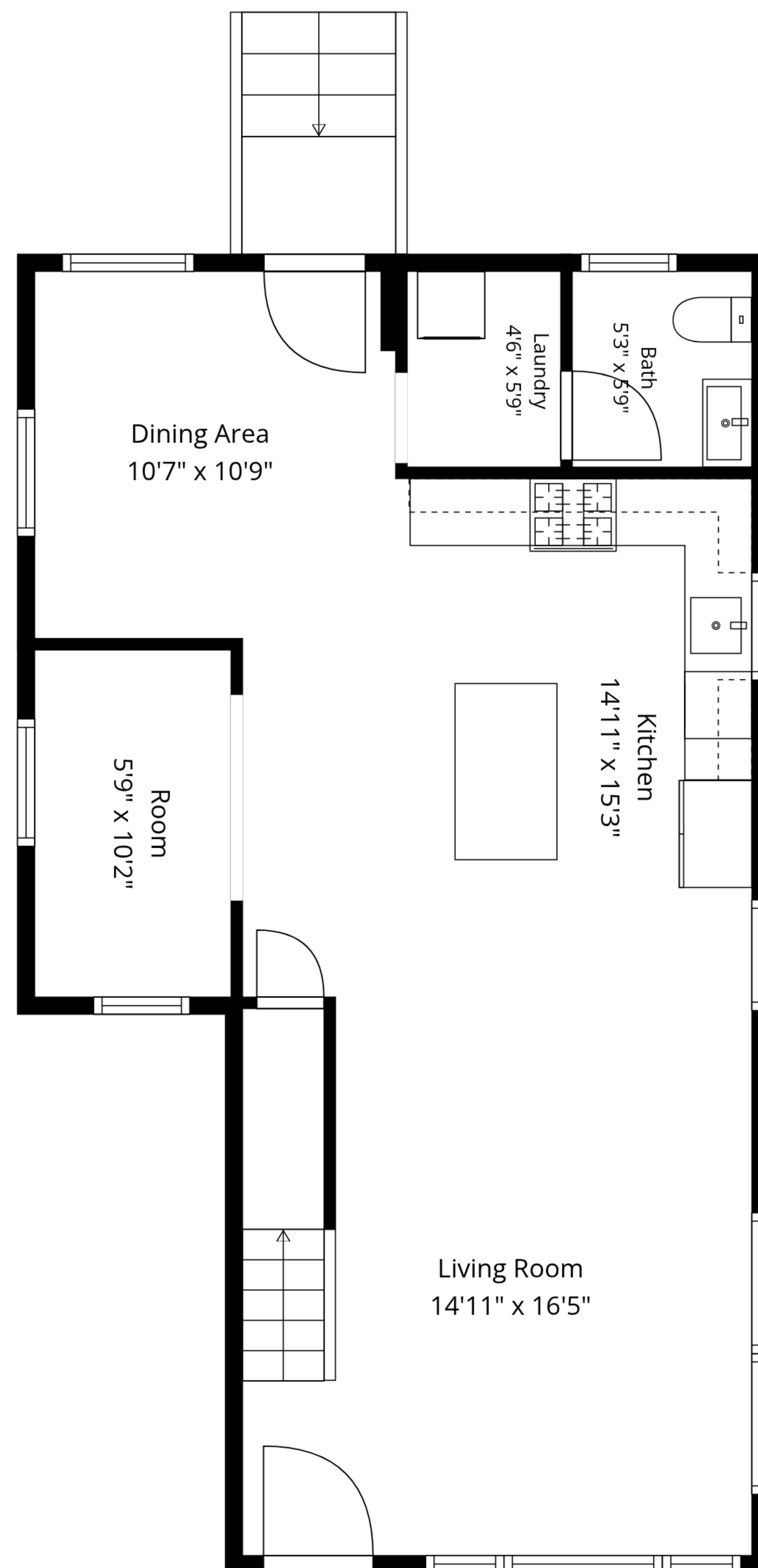
1st Floor
