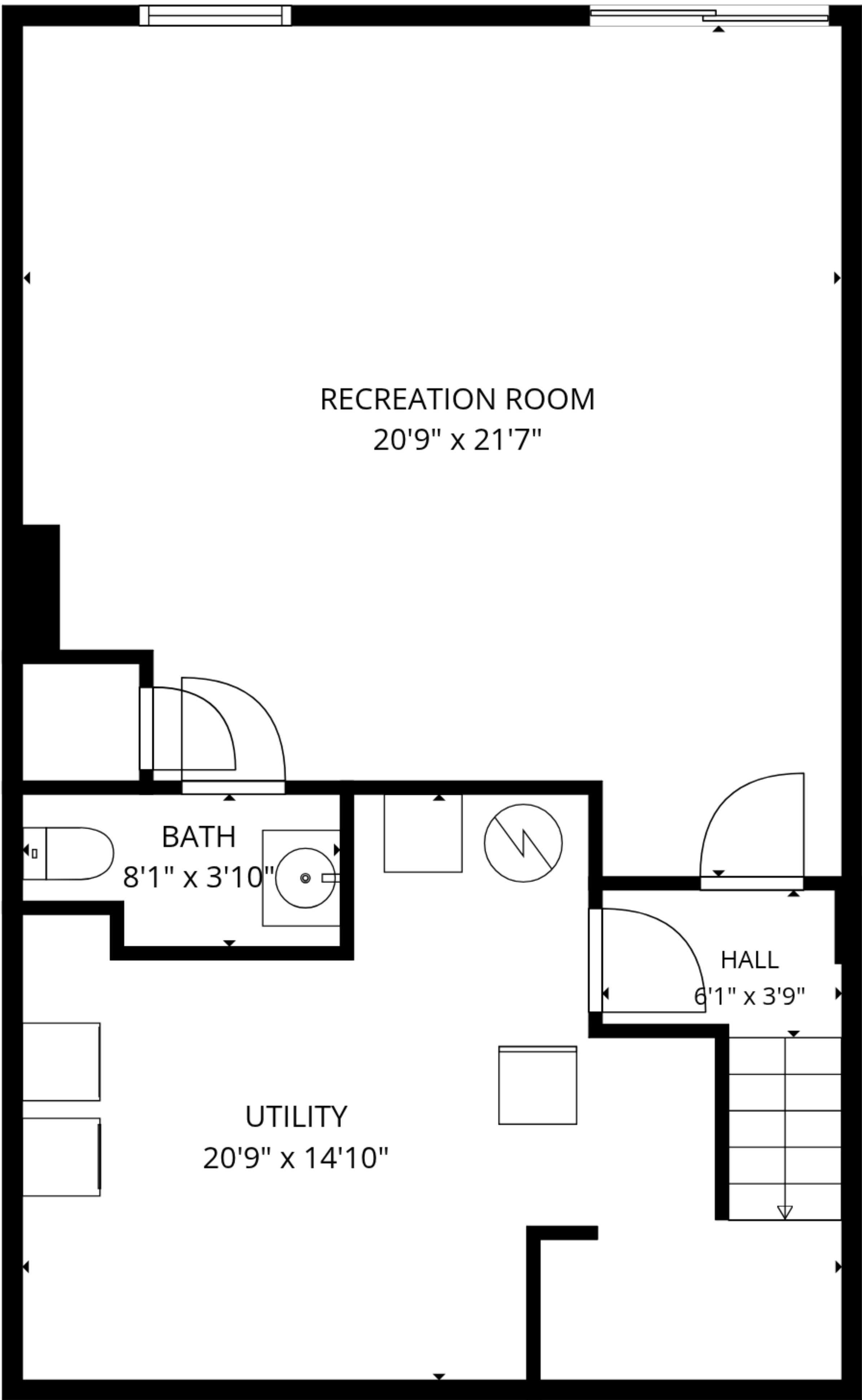
Basement
