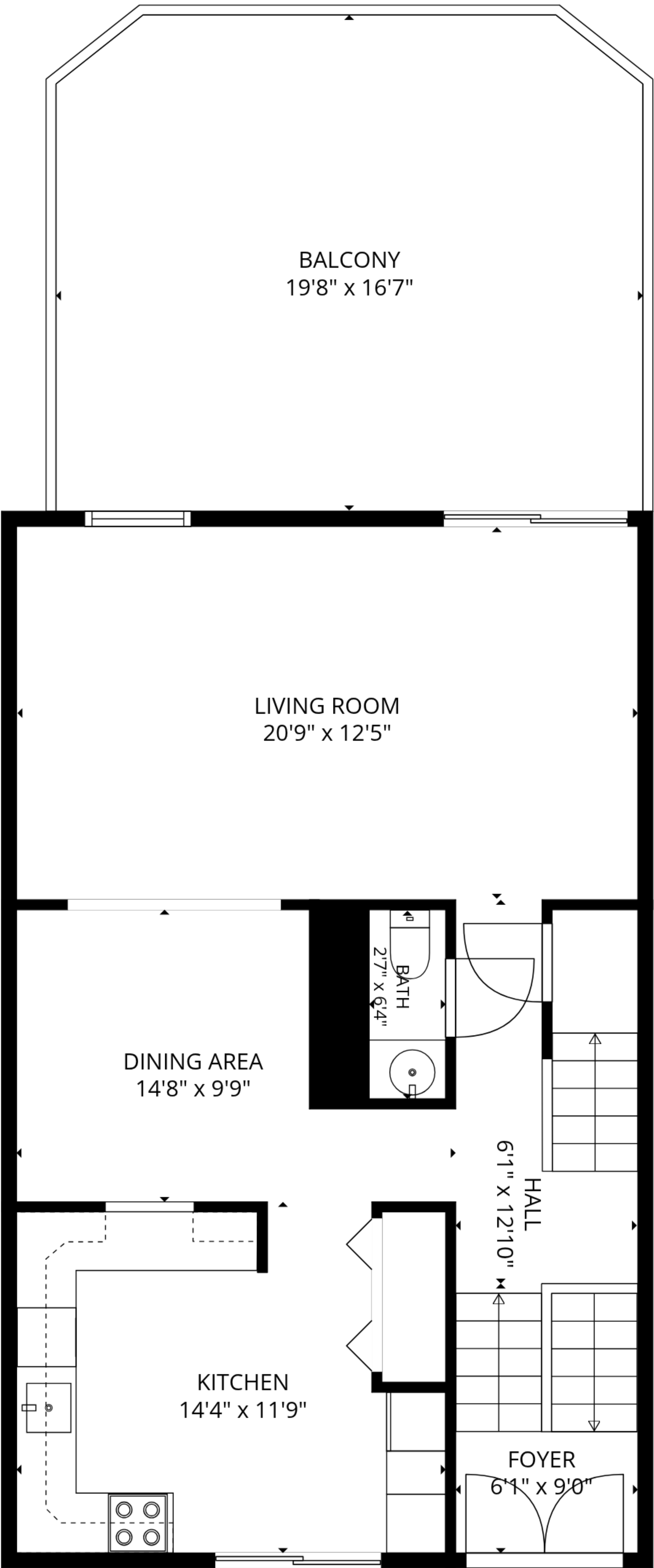
1st floor
