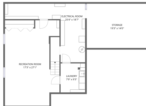
Basement
