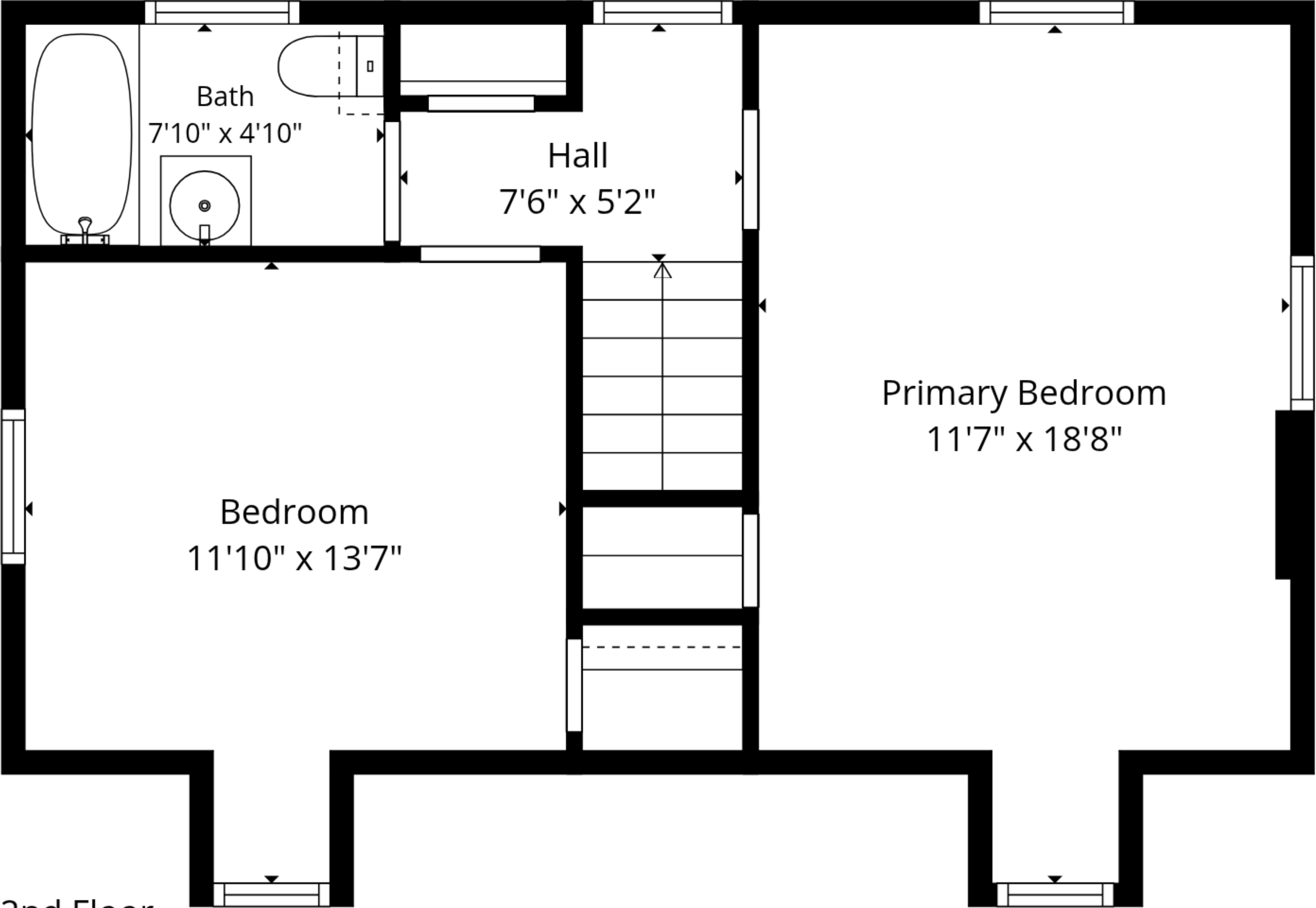
2nd Floor
