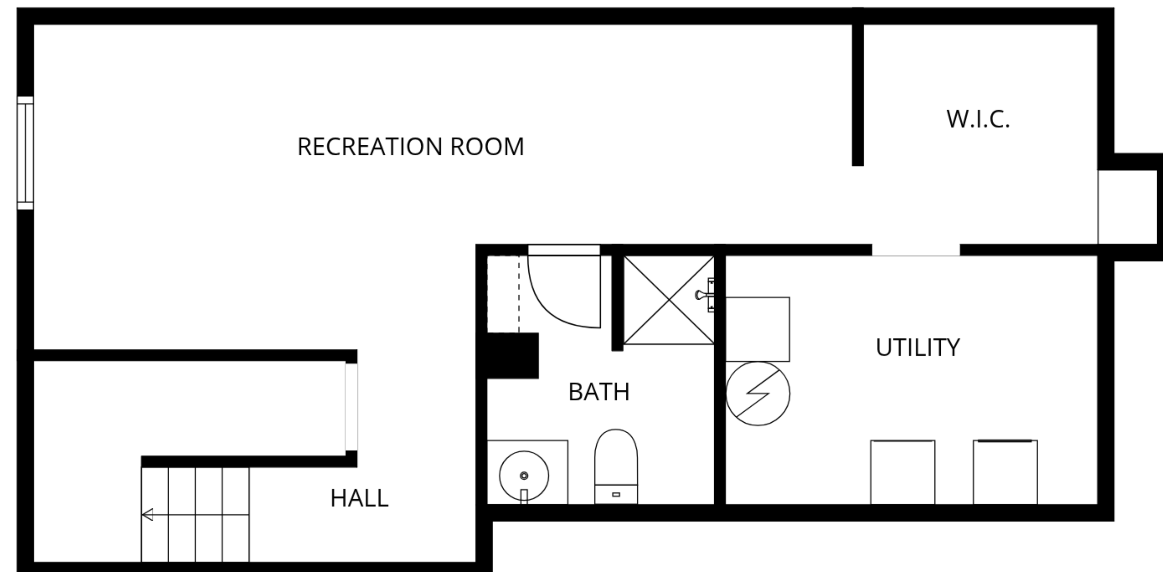
FLOOR 1
