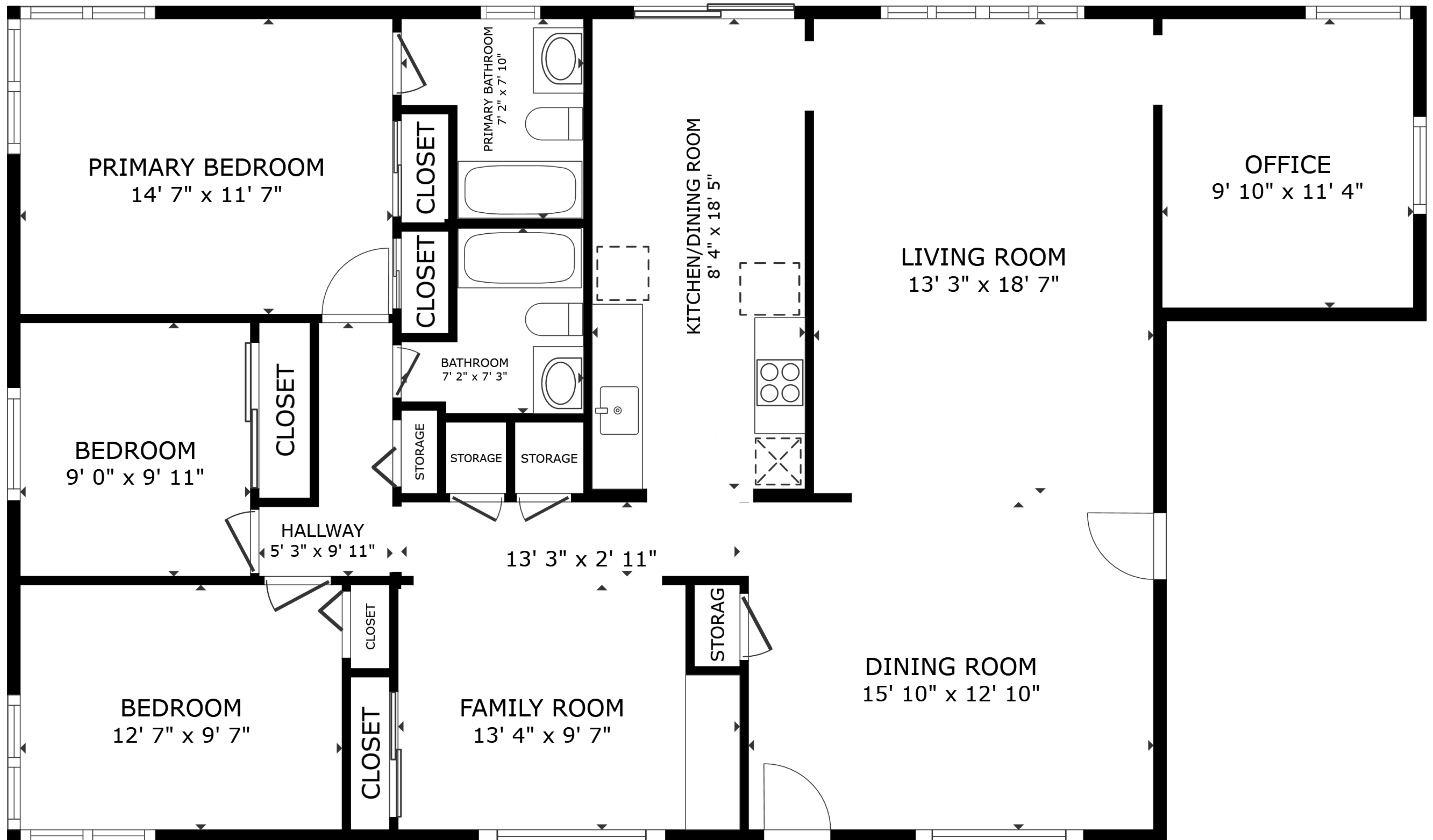
FLOOR PLAN
