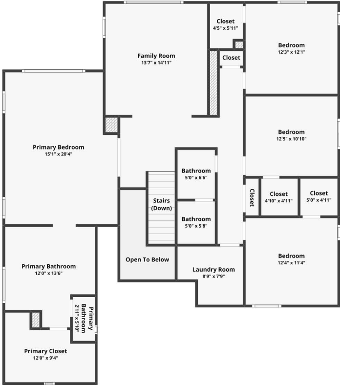
FLOOR 2 Finished area: ~1,556.72 sq. ft.
