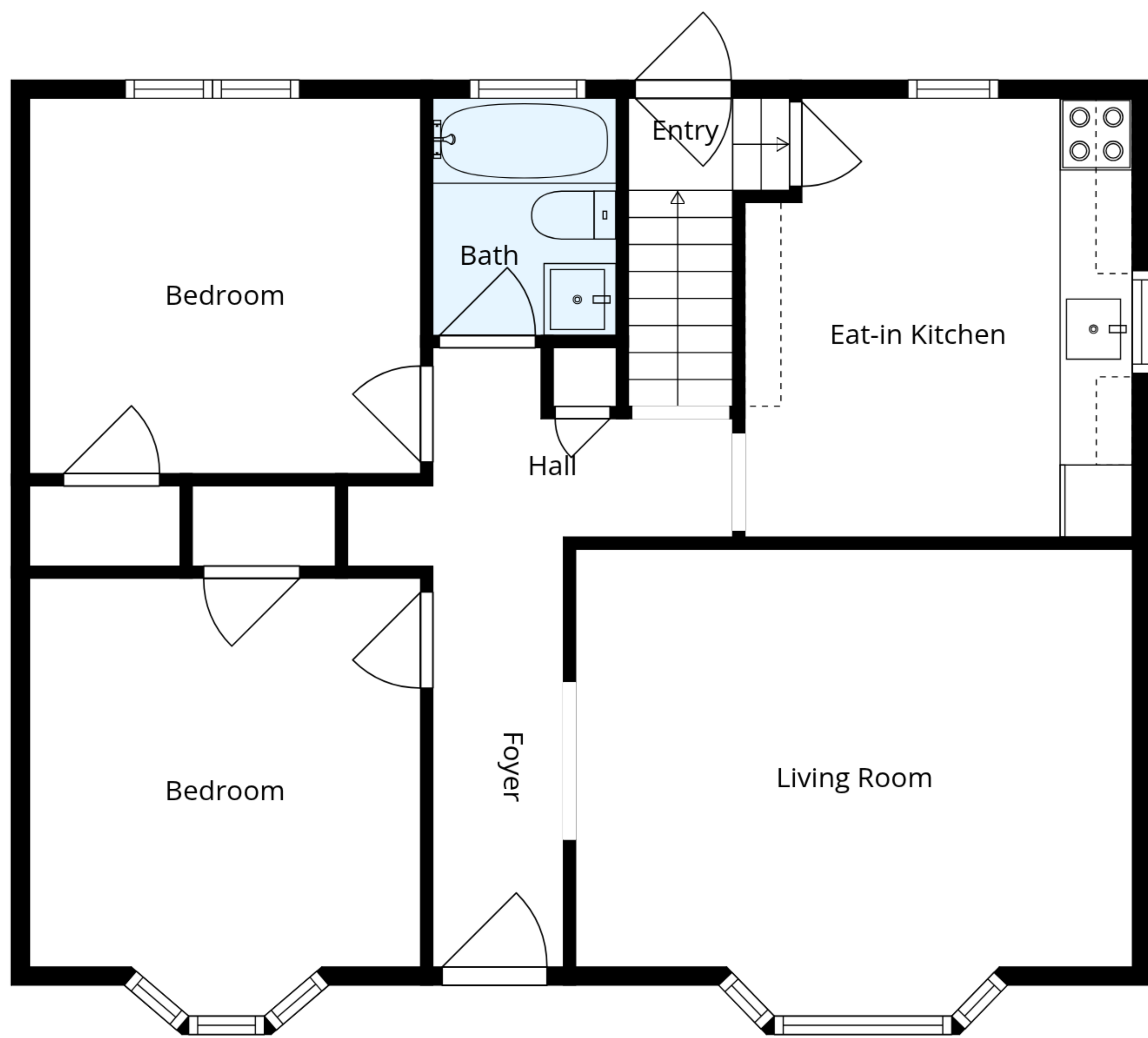
1st Floor
