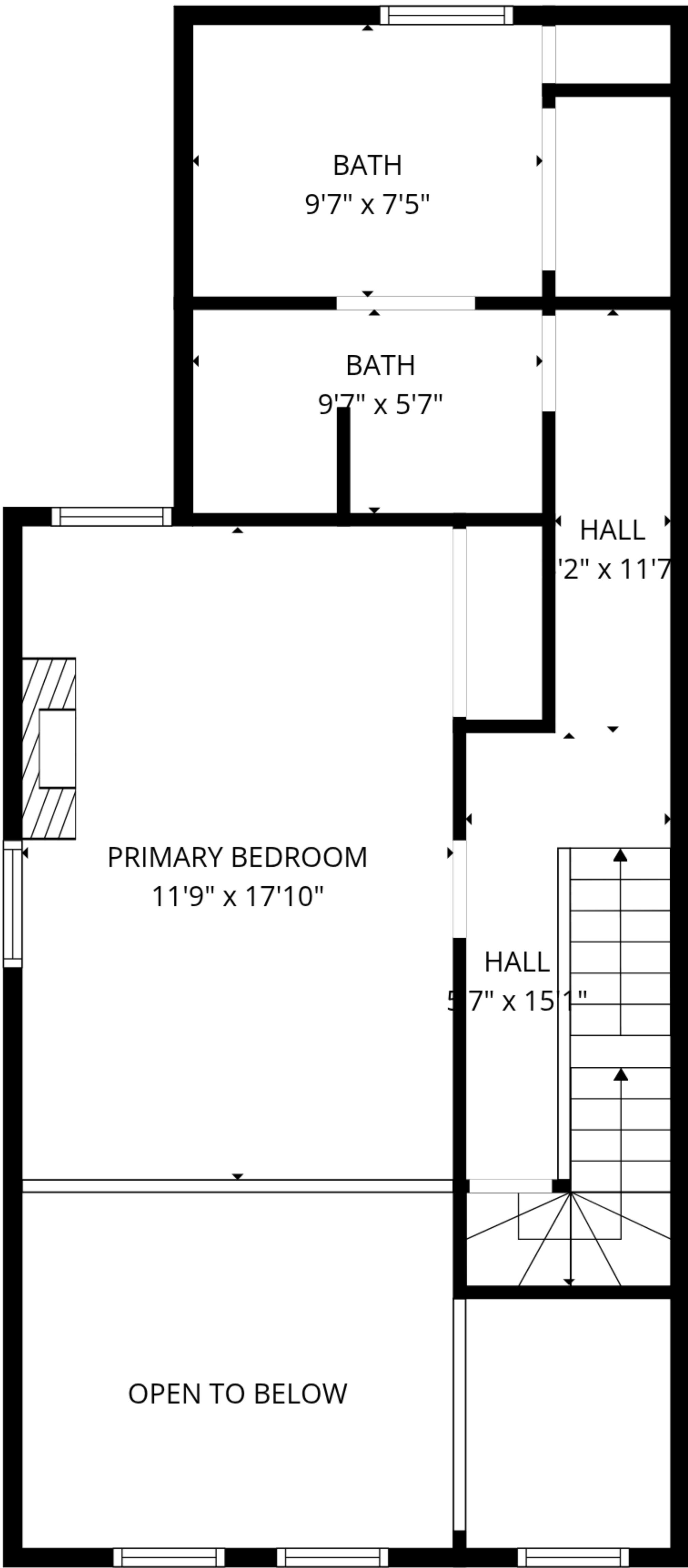
2nd floor
