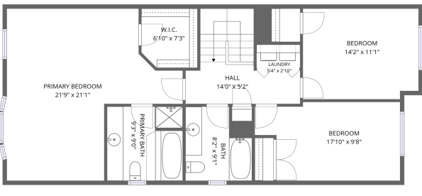
2nd floor
