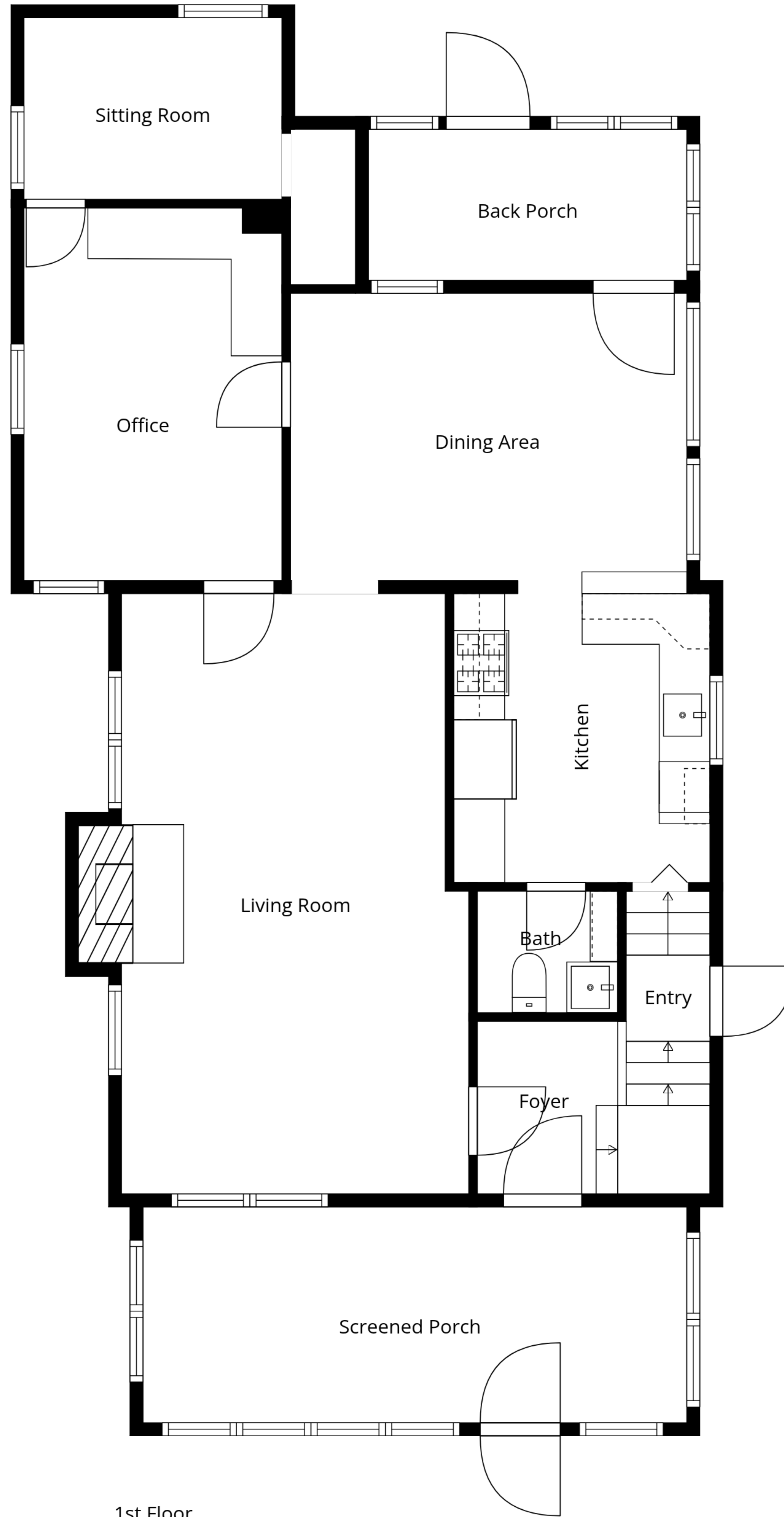
1st Floor
