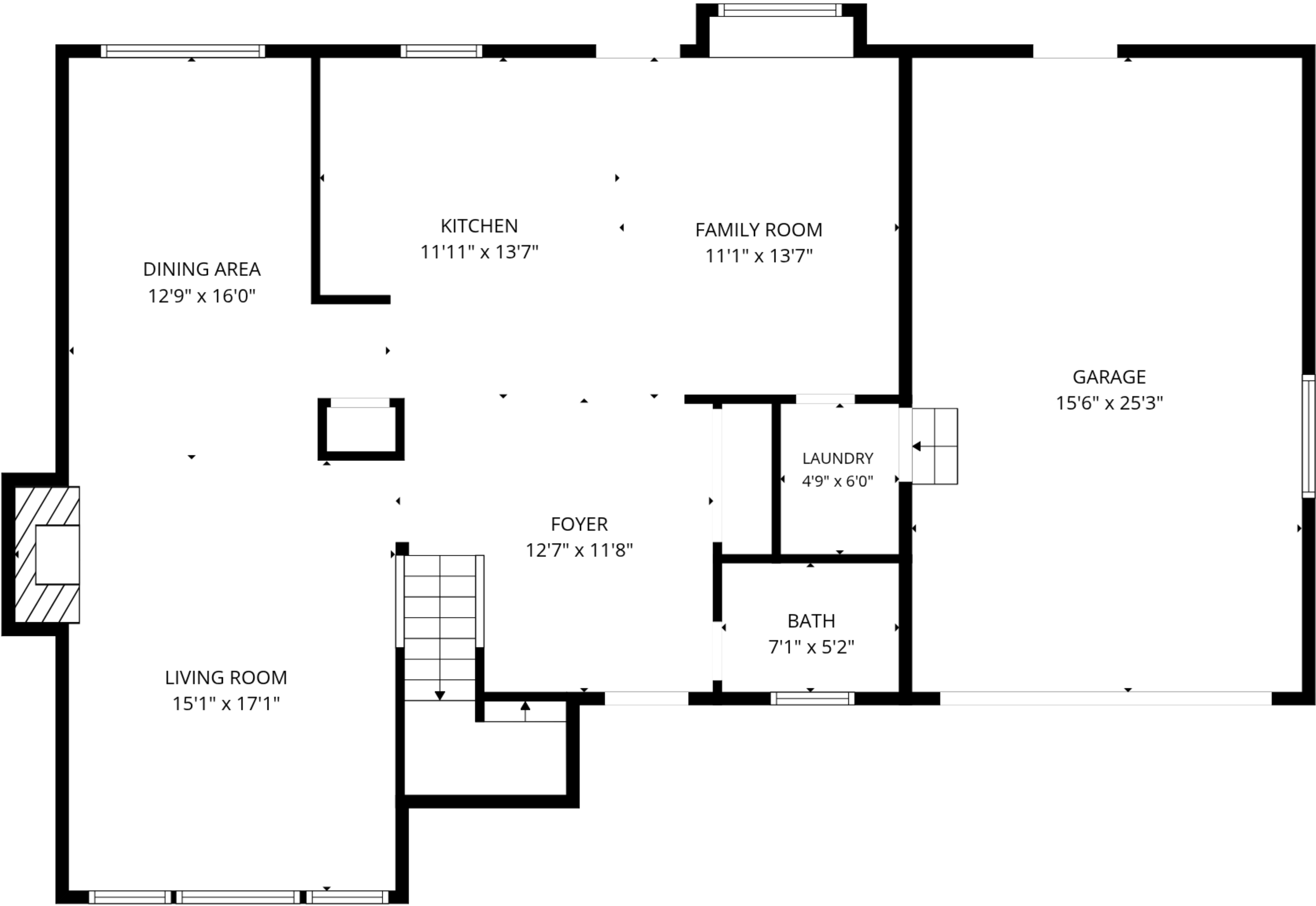
1st floor
