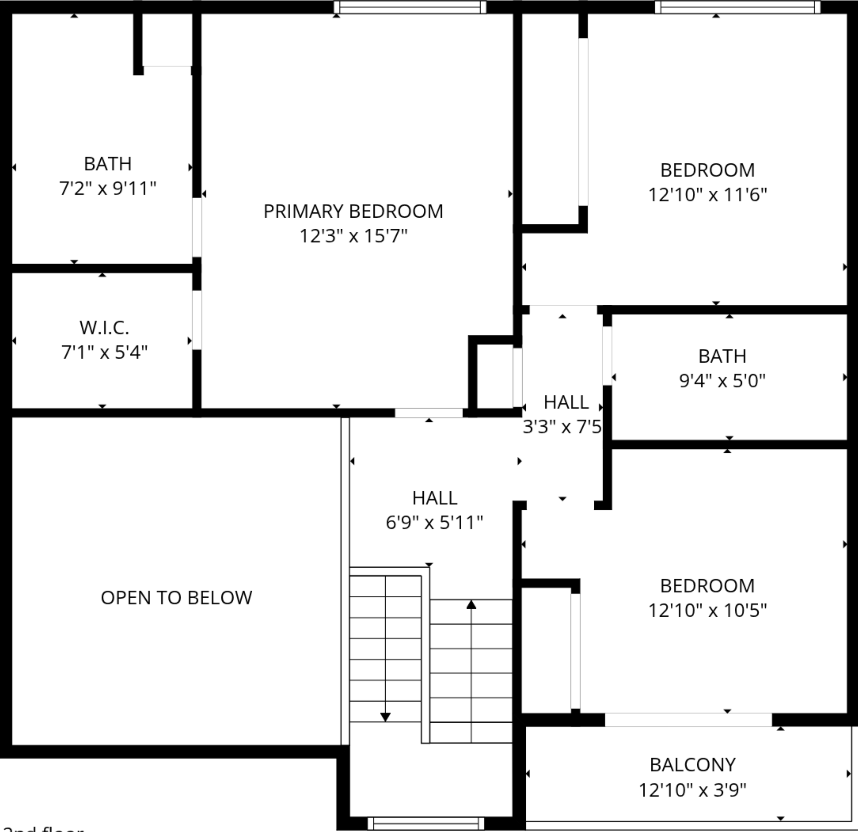
2nd floor
