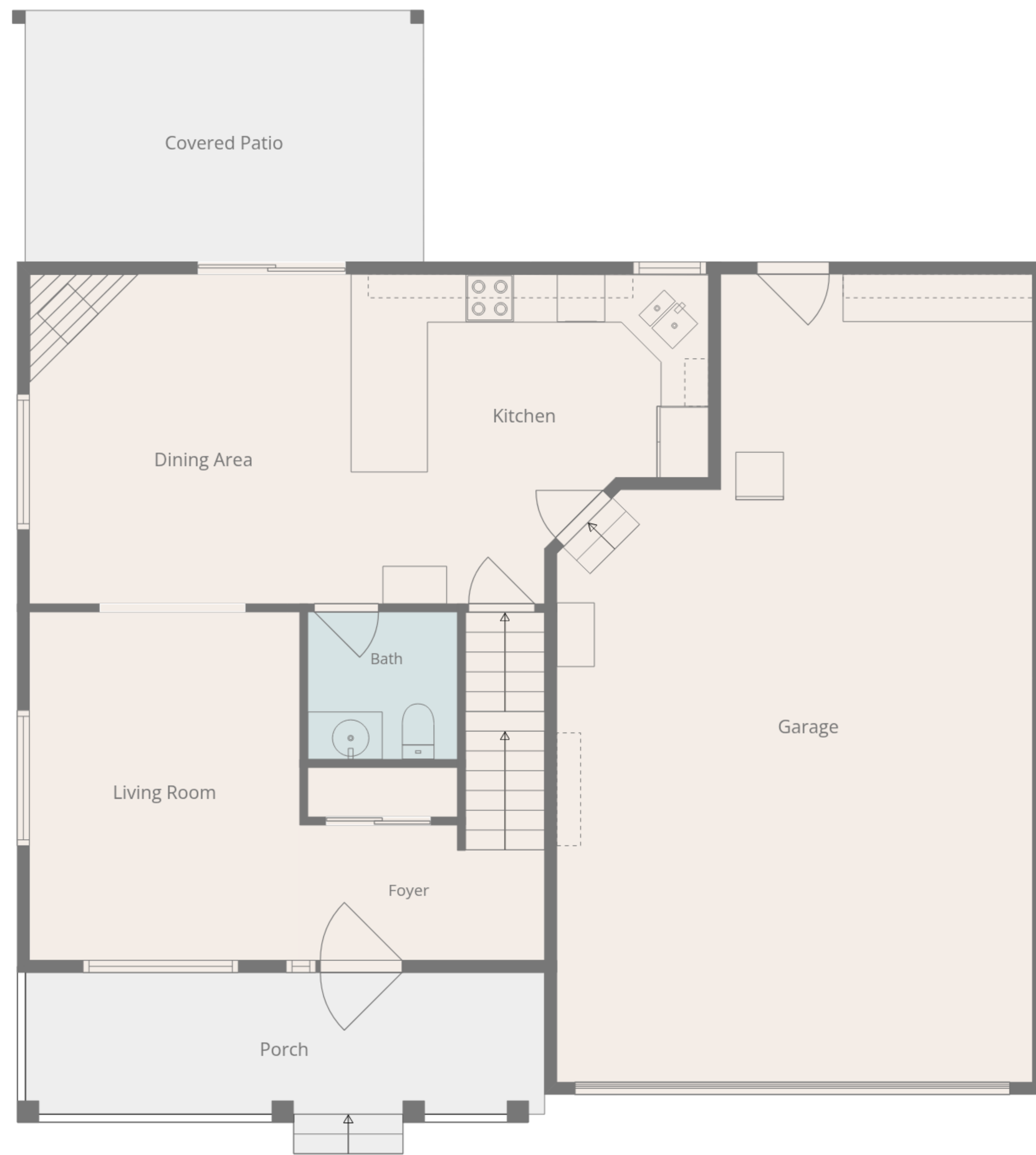
1st Floor
