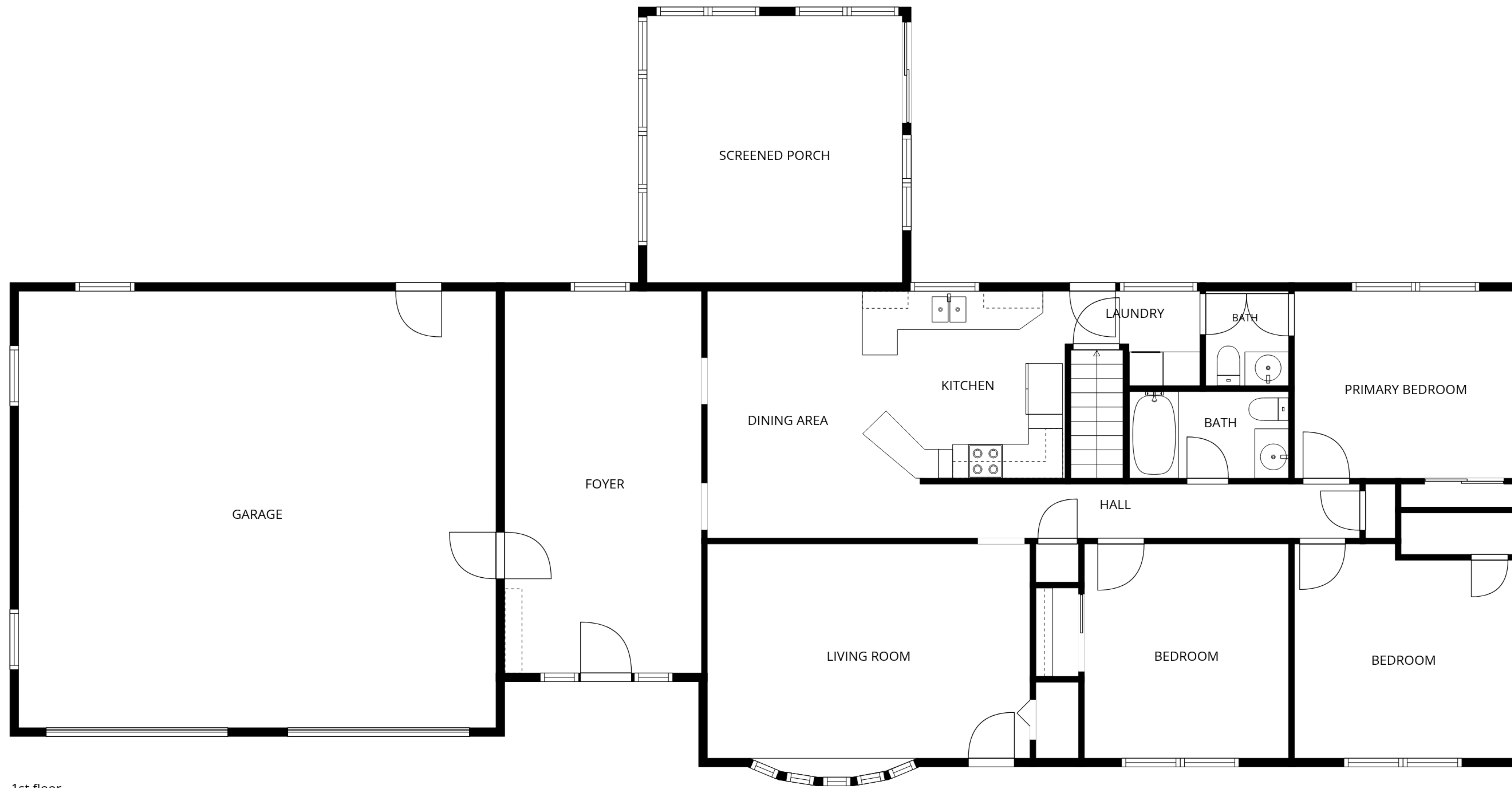
1st floor
