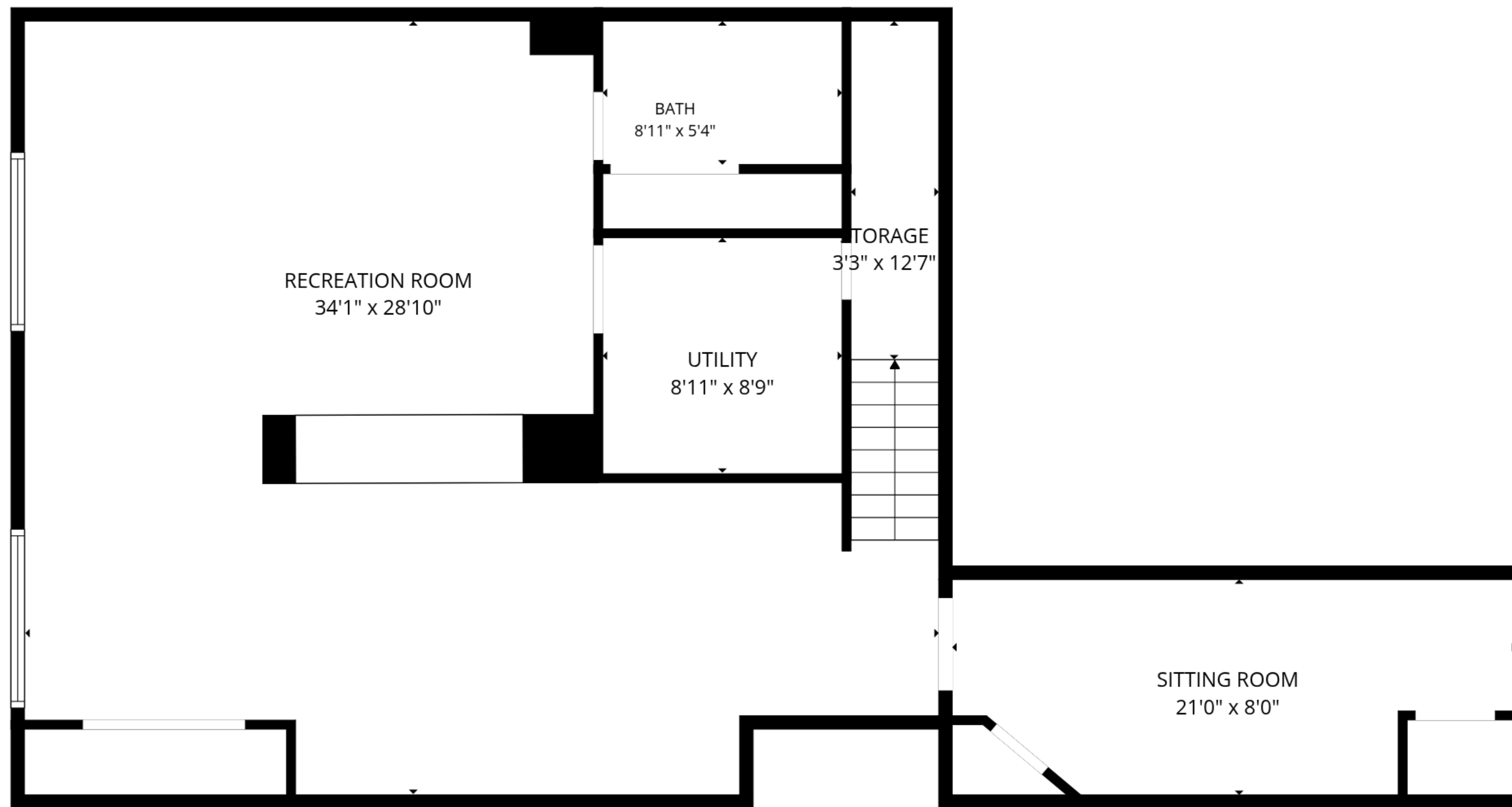
Basement
